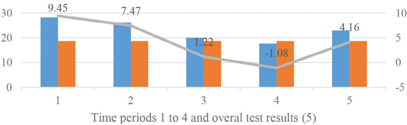
Figure 8: Comparison of energy performance gap with design values of all variables except n_{50} (measured value of 5.19 \text{ h}^{-1} was taken) (Test 2).
