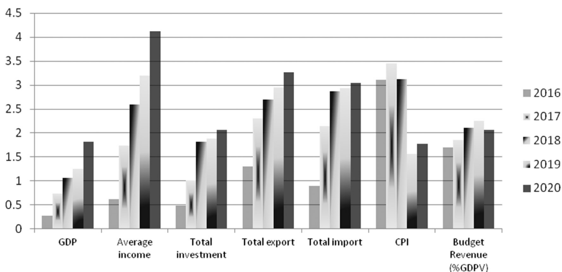
Fig. 2. Target scenario forecasts vs. Baseline scenario ones (% point)
