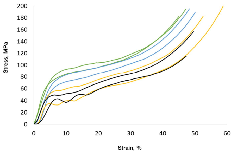
Fig. 1. Stress-strain diagram to determine the characteristic values from compression testing of porous samples under different preparation protocol (after SLM only - green; annealing at 625°C - blue; annealing at 675°C - yellow, annealing at 725°C - black).
