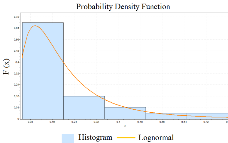
Figure 1: Approximation of the \varphi_i values distribution by means of a lognormal distribution function.
