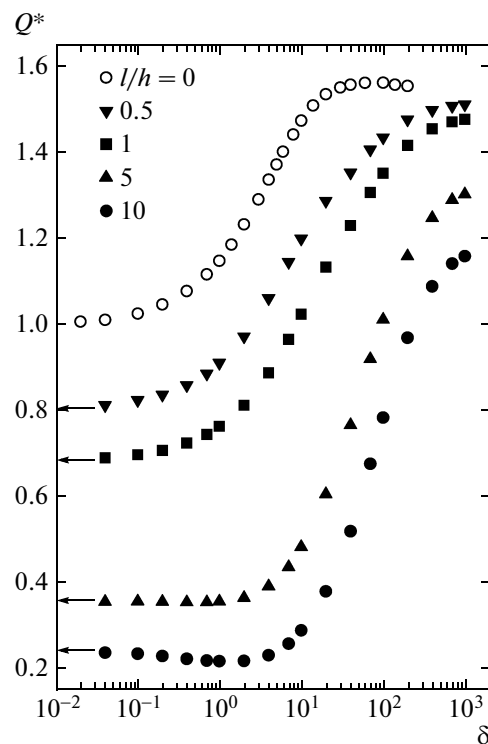
Fig. 2a. The dimensionless mass flow rate Q^* as a function of gas rarefaction parameter \delta for various reduced channel length l/h .
