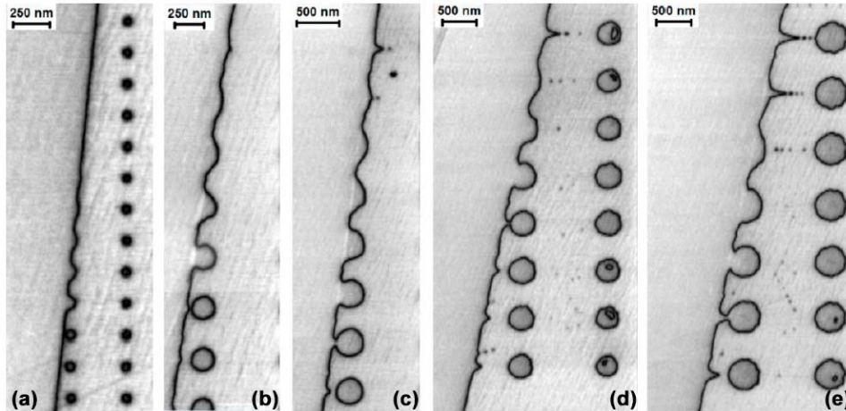
Figure 2. Tip-induced switching in contact mode in LiNbO 3 single crystal near flat domain wall with different amplitudes of the switching pulses: (a) 20 V; (b) 40 V; (c) 60V; (d) 80V and (e) 100 V. PFM amplitude signal.
