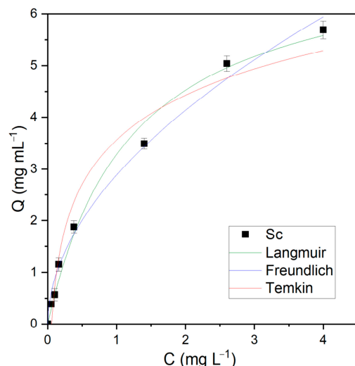
Figure 2. Langmuir, Freundlich, and Temkin adsorption isotherms obtained for Sc adsorption on MTS9580 from simulated sulfuric acid solutions at pH 3.5.
