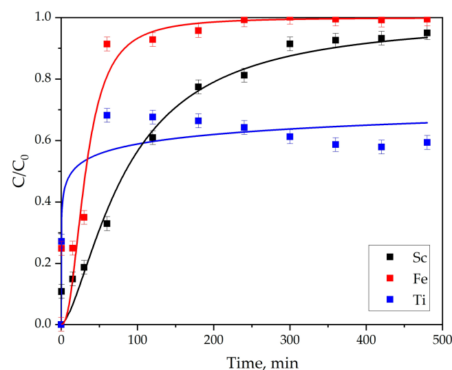
Figure 4. MDR model column adsorption on MTS9580 at PLS flow rate of 7.5 mL min −1 .
