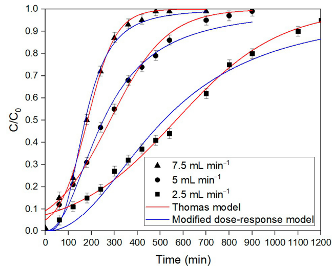
Figure 3. Column adsorption of Sc from a simulated solution on MTS9580 at flow rate of 2.5–7.5 mL min −1 .
