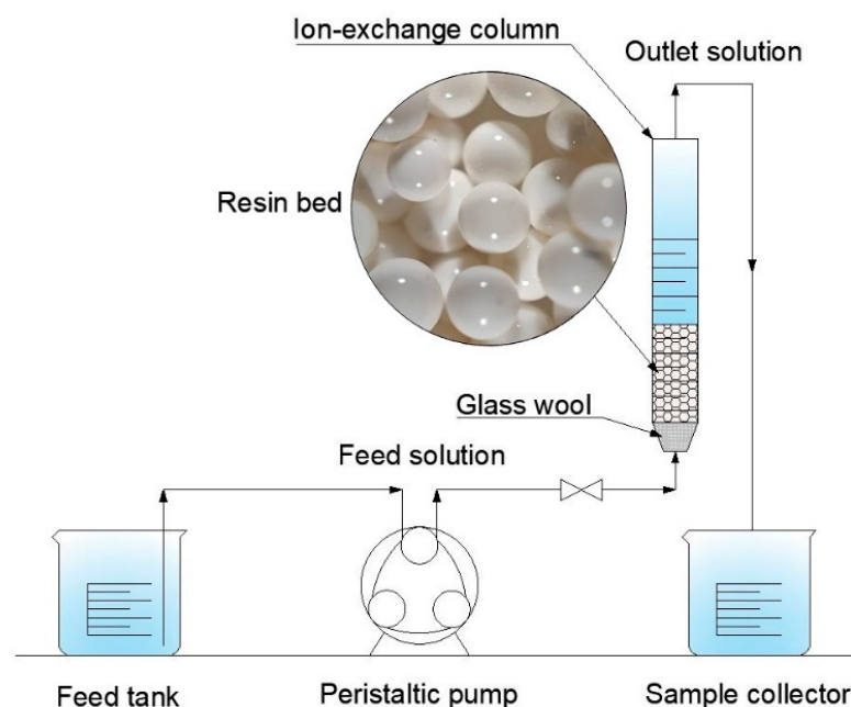
Figure 1. The column ion-exchange experimental unit.
