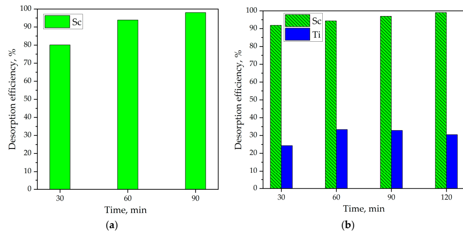
Figure 5. Desorption efficiency with \text{NaHCO}_3 solution ( 200 \text{ g L}^{-1} ) from MTS9580, saturated using a model solution (a); PLS (b).
