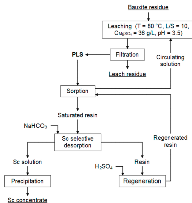
Figure 6. The principal flowsheet of Sc concentrate obtained from PLS using Puromet MTS9580 ion-exchange sorption.
