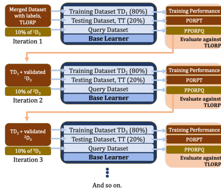
Figure 4. A schematic overview of the self-training semi-supervised learning mechanism using base learners. These base learners can be linear (e.g., find linear patterns only) or non-linear models (e.g., finds linear and non-linear patterns).
