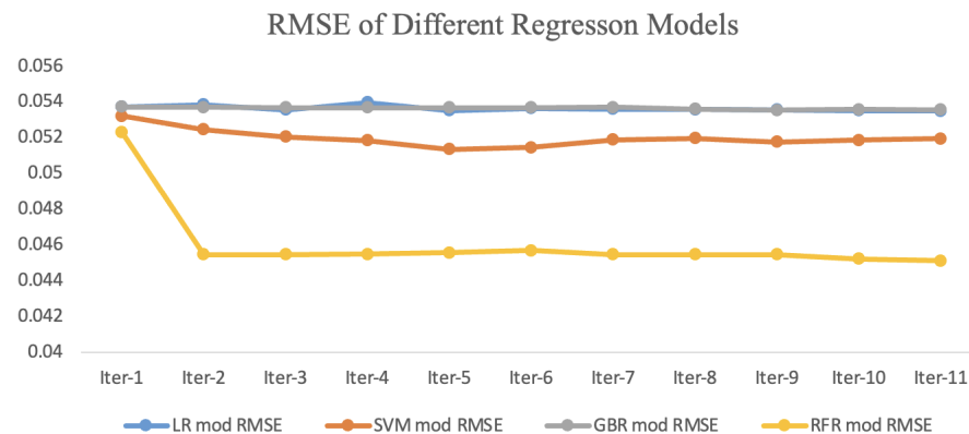
Figure 8. The RMSE values of the four ML regression models over the ten iterations of the self-training stage plus the initially supervised base learner.
