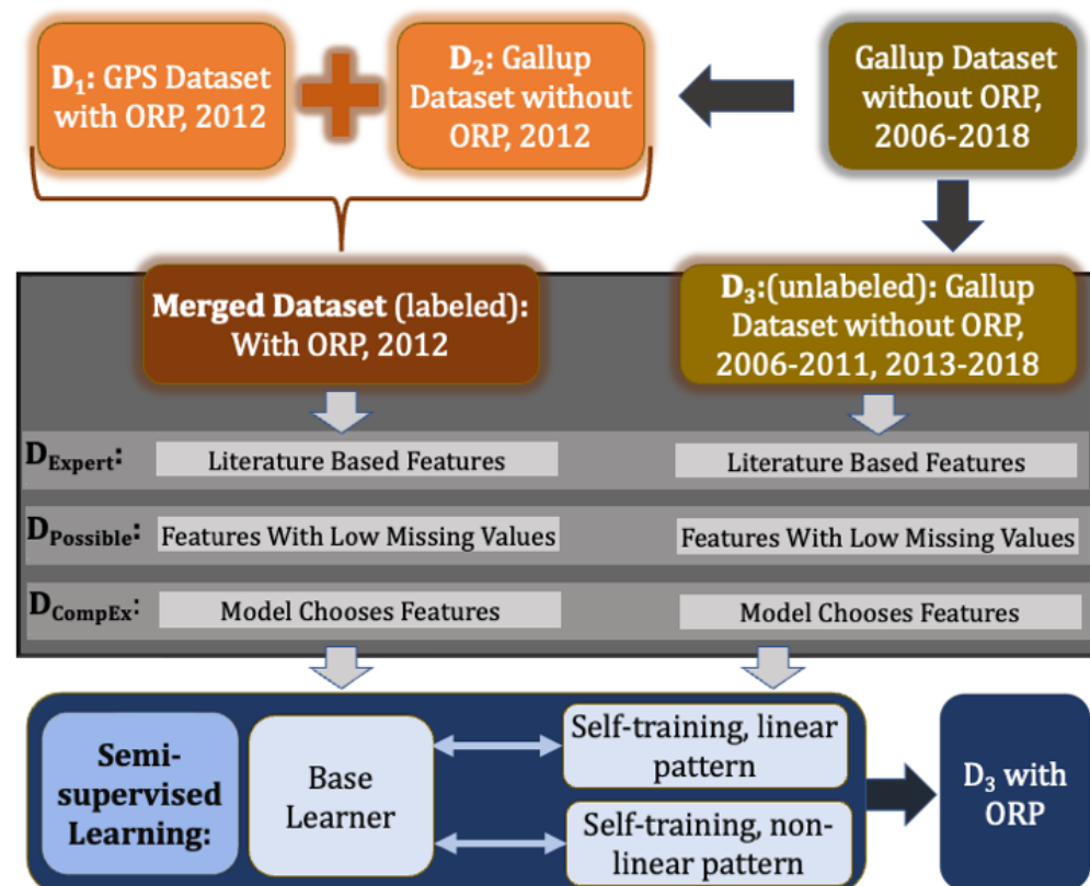
Figure 1. An overview of the research methodology used to predict ORP values for the Gallup data.
