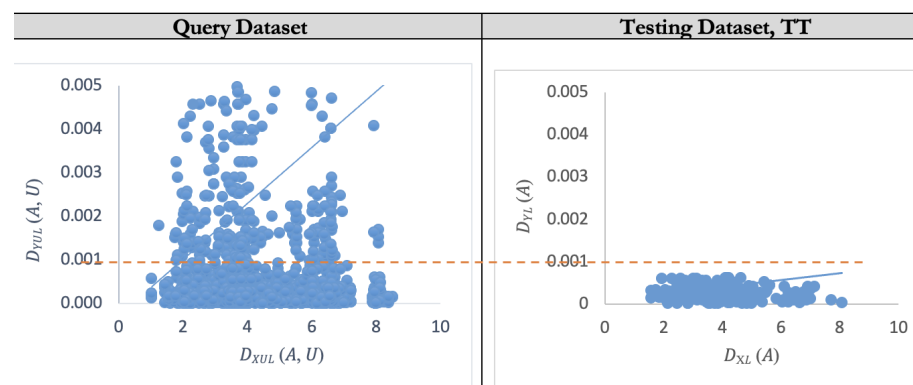
Figure 7. Scatter plot comparison for LR Self-training, first iteration, Step 1 (left) and Step 2 (right). This particular figure uses the D_{Expert} dataset.
