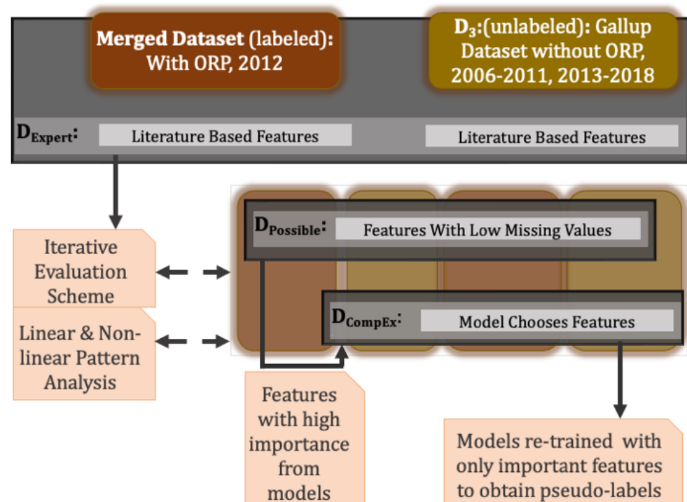
Figure 2. An overview of the data usage and the contributions of this research work.
