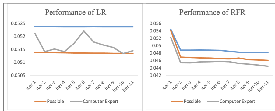
Figure 9. The performance of the LR and RFR model on the three datasets, D_{Expert} , D_{Possible} , D_{CompEx} . The best regression prediction is by RFR on D_{CompEx} .
