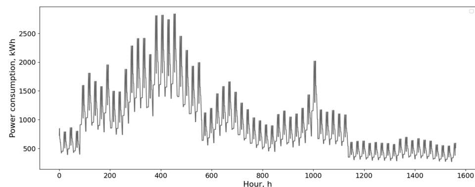
Figure 3. Actual power consumption of compressor station from December 2020 to January 2021.
