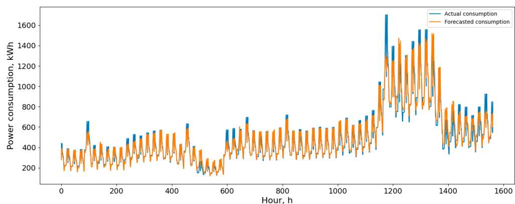
Figure 11. Actual and forecast power consumption from September 2020 to October 2021.
