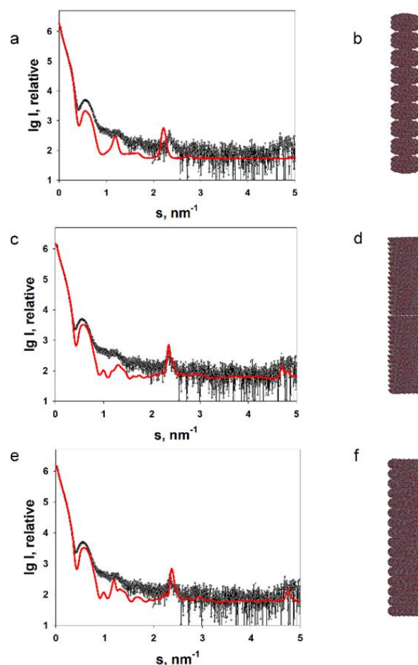
Figure 1. Experimentally obtained SAXS profile of repolymerized TMV CP stacked discs (a,c,e) and calculated SAXS data for the corresponding model structures (b,d,f). The scattering was calculated using the CRY SOL program. The structures of the replicated crystallographic model (b), the lower pair of discs (d) and the central pair of discs (f) were modelled with the MASSHA program. Points, experimental data; solid lines, calculated scattering of the model structures. Reprinted from [58], Copyright (2020), with permission from Springer Nature.
