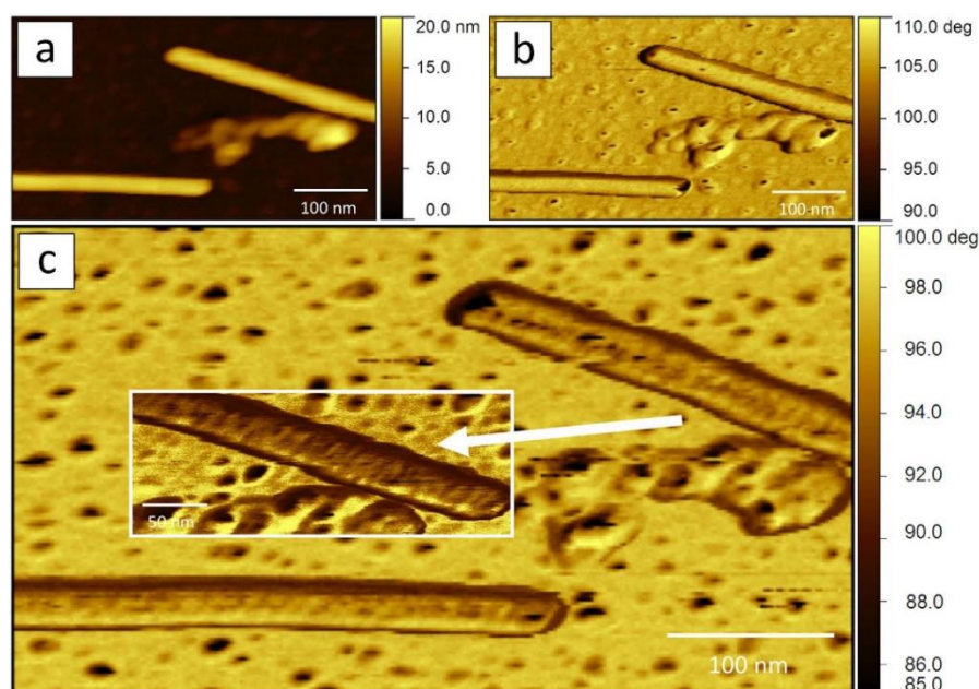
Figure 5. Standard and multi-frequency AFM images of TMV virions: (a) height image; (b) phase shift image of the first excited mode (115 kHz); (c) phase shift image of the second excited mode (720 kHz). Reproduced from [72] under the CC BY license ( https://creativecommons.org/licenses/by/4.0/ (accessed on 7 March 2024)).
