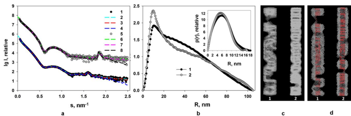
Figure 3. (a) Curves 1 and 5 are the experimental ones; curves 2 and 6 were calculated with the GNOM program based on the distance distribution functions p(r) ; curves 3 and 7 are the scattering profiles calculated from the ab initio models reconstructed with the DAMMIN program; curves 4 and 8 are scattering profiles calculated from the multiphase ab initio models reconstructed with the MONSA program for PVA and PVA \Delta 32, respectively. For better visualization the scattering curves from PVA and PVA \Delta 32 are shifted vertically relative to each other; (b) calculated with GNOM program distance distribution functions from PVA (1) and PVA \Delta 32 (2). Inset: distance distribution functions p(r) in the cross-sectional analysis mode calculated for PVA (1) and PVA \Delta 32 (2); (c) shapes of PVA (1) and PVA \Delta 32 (2) virions reconstructed with the DAMMIN program; (d) shapes of PVA (1) and PVA \Delta 32 (2) virions reconstructed with the MONSA program. Protein coat is presented as grey virtual atoms (beads), viral RNA—as red beads. Reprinted from [60], copyright (2021), with permission from Springer Nature.
