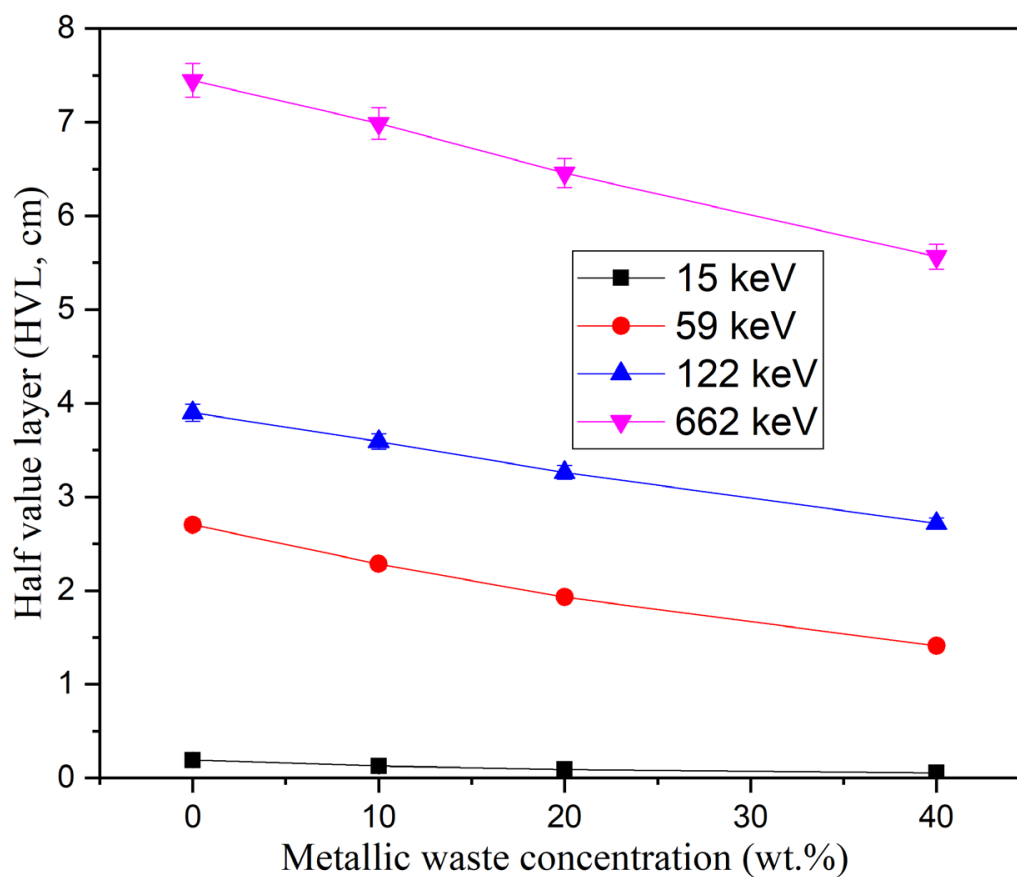
Figure 8. Dependence influence of the heavy metallic waste concentrations on half-value thickness ( \Delta 0.5 , cm) at some fixed \gamma -photon energy.
