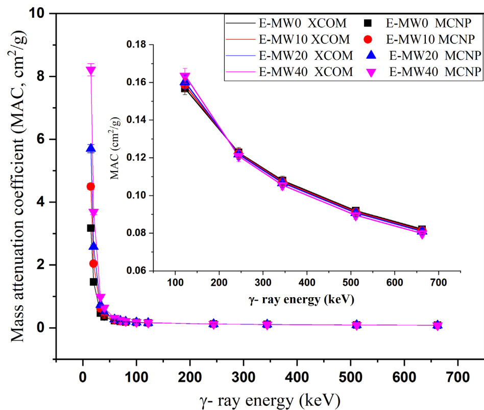
Figure 3. Mass attenuation coefficient variation of the fabricated samples vs. incident gamma energy of photons at photon energy.
