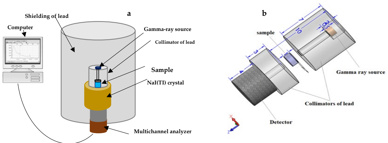
Figure 1. (a) Diagram illustrating the procedure of measuring the linear attenuation coefficient using the narrow beam transmission technique and (b) a three-dimensional representation of the MCNP-5 input file.
