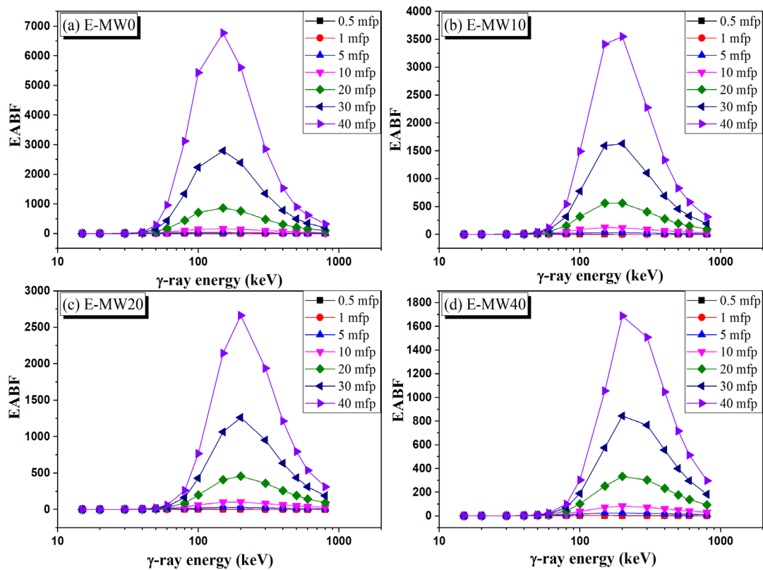
Figure 12. Dependence of absorption buildup factor (EABF) on the \gamma -photon energy.
