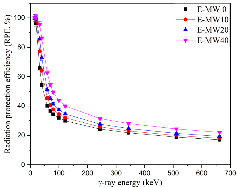
Figure 4. Variation of dependence of the radiation protections efficiency (RPE, %) on the \gamma -photon energy.
