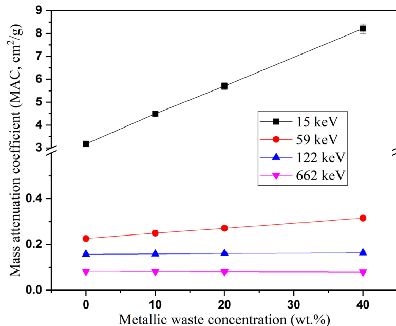
Figure 7. Reliance impact of weight percentage concentrations of metallic waste on the mass attenuation coefficient at a given \gamma -photon energy.
