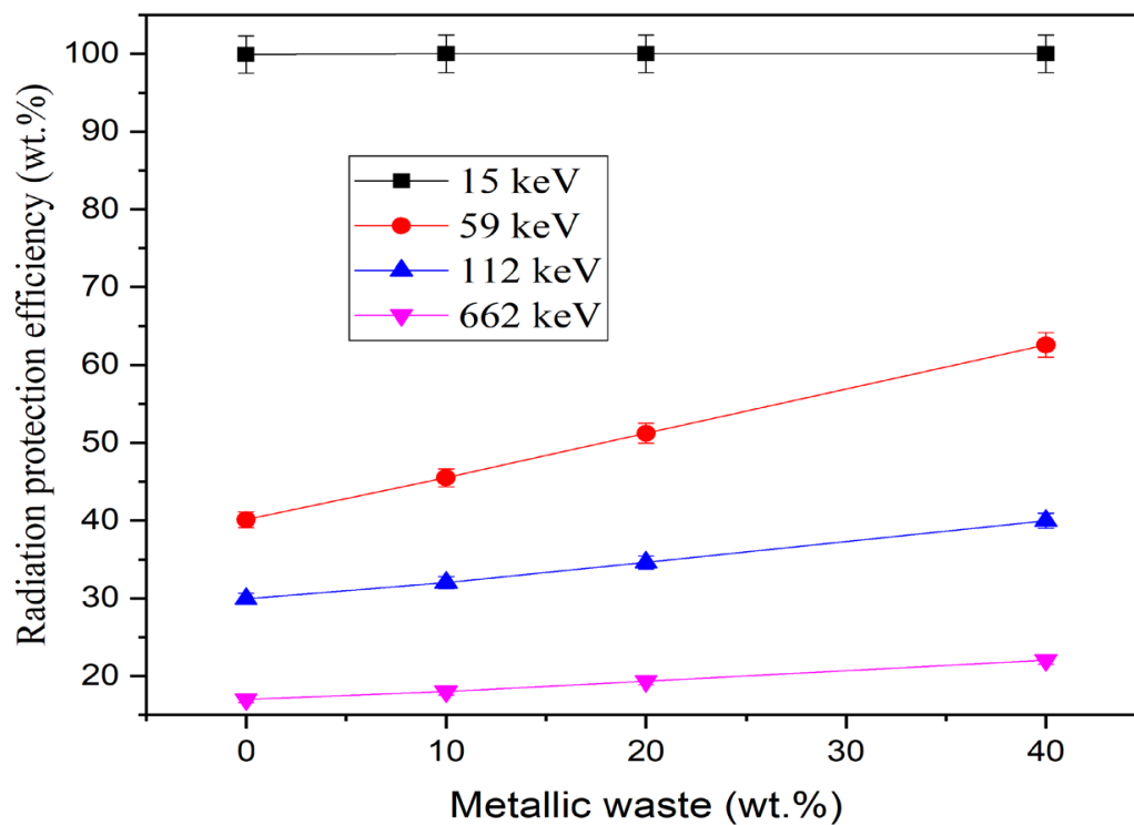
Figure 9. The fabricated composites' radiation protection effectiveness (RPE, %) as a function of metallic waste.
