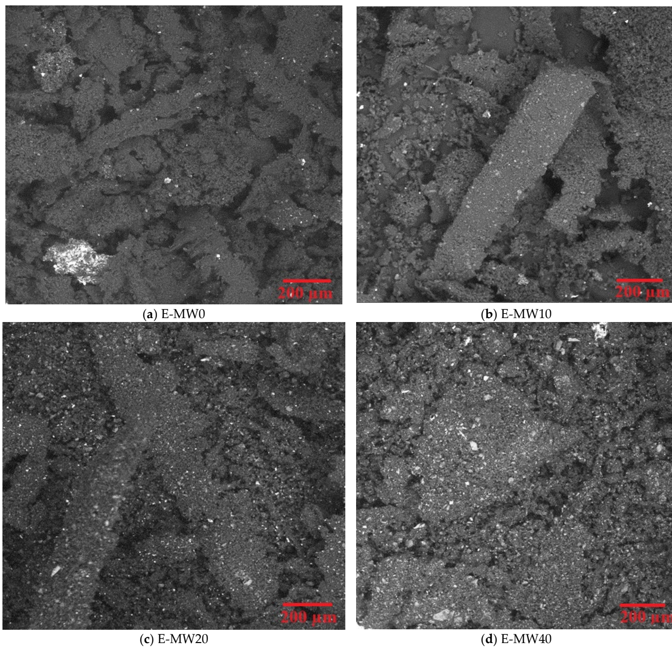
Figure 2. SEM images for the E-MW0, E-MW10, E-MW20, and E-MW40 fabricated samples.
