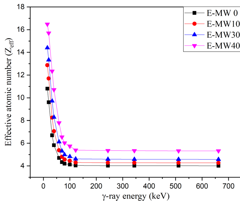
Figure 5. Relationship between the effective atomic number ( Z_{eff} ) and the energy of \gamma -photon.
