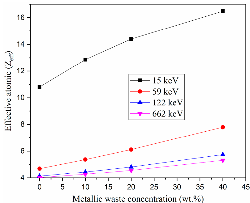
Figure 6. Dependence of effective atomic number ( Z_{eff} ) on the metallic waste concentration.
