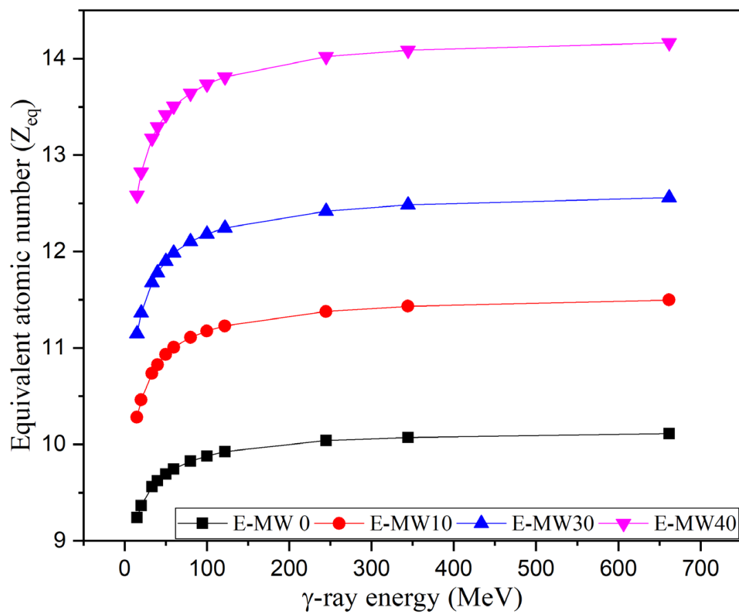
Figure 10. The relationship between the \gamma -photon energy and the equivalent atomic number ( Z_{eq} ).
