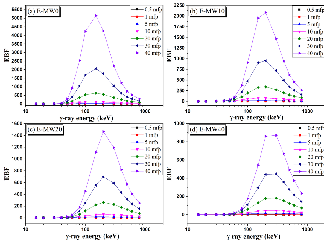
Figure 11. Dependence of exposure buildup factor (EBF) on the \gamma -photon energy.
