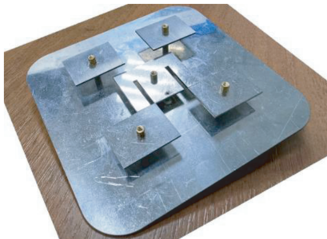
FIGURE 10. The prototype of the proposed wideband antenna based on an E-shaped active exciter.
