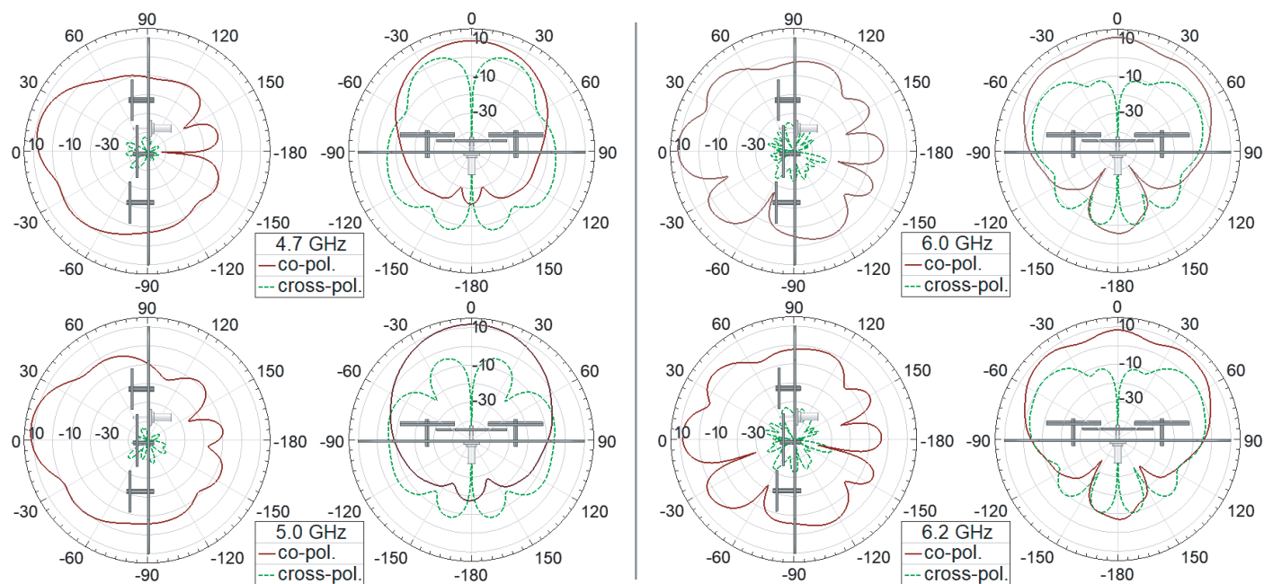
FIGURE 8. The simulated gain patterns of the antenna with an E-shaped active exciter and four rectangular passive elements.
