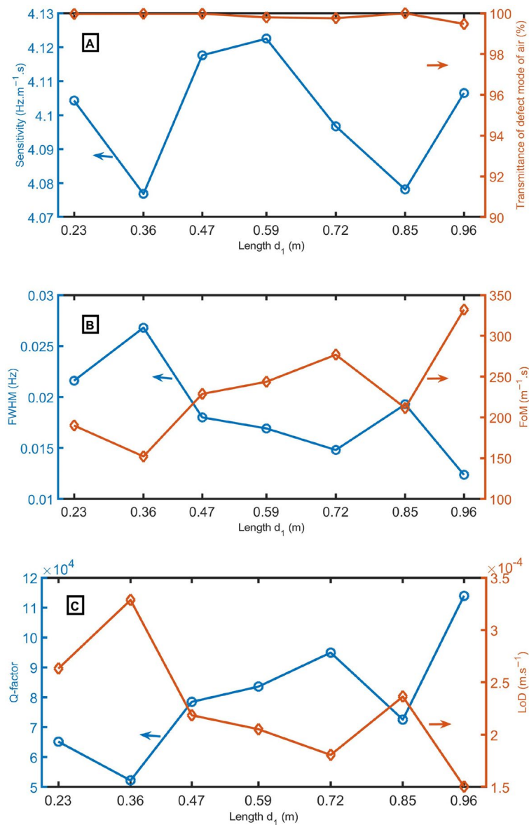
Figure 11. (A) sensitivity and transmittance intensity, (B) FWHM of defect mode for air sample and FoM, and (C) Q-factor and LoD as a function of length d_1 at N = 12 periods, d_1 = 0.6 m, d_D = 1.3 m, d_2 = 0.15 m, S_1 = 1 m 2 , S_D = 0.75 m 2 , and S_2 = 0.75 m 2 .
