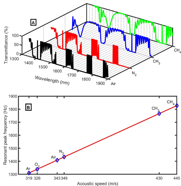
Figure 13. (A) The transmittance spectra of the closed resonator system, and (B) the resonant peak position versus acoustic speeds using different gas samples at optimum conditions at N=12 , d_l=0.96 m, S_l=1 m 2 , d_2=0.15 m, S_2=0.75 m 2 , S_D=0.75 m 2 , and d_D=1.3 m.
