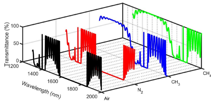
Figure 3. The transmittance spectra of the closed resonator system using different gas samples at d_i = 0.6 m, N = 10 , d_2 = 0.15 m, S_i = 1 m 2 , d_D = 0.45 m, S_D = 0.73 m 2 , and S_2 = 0.75 m 2 .
