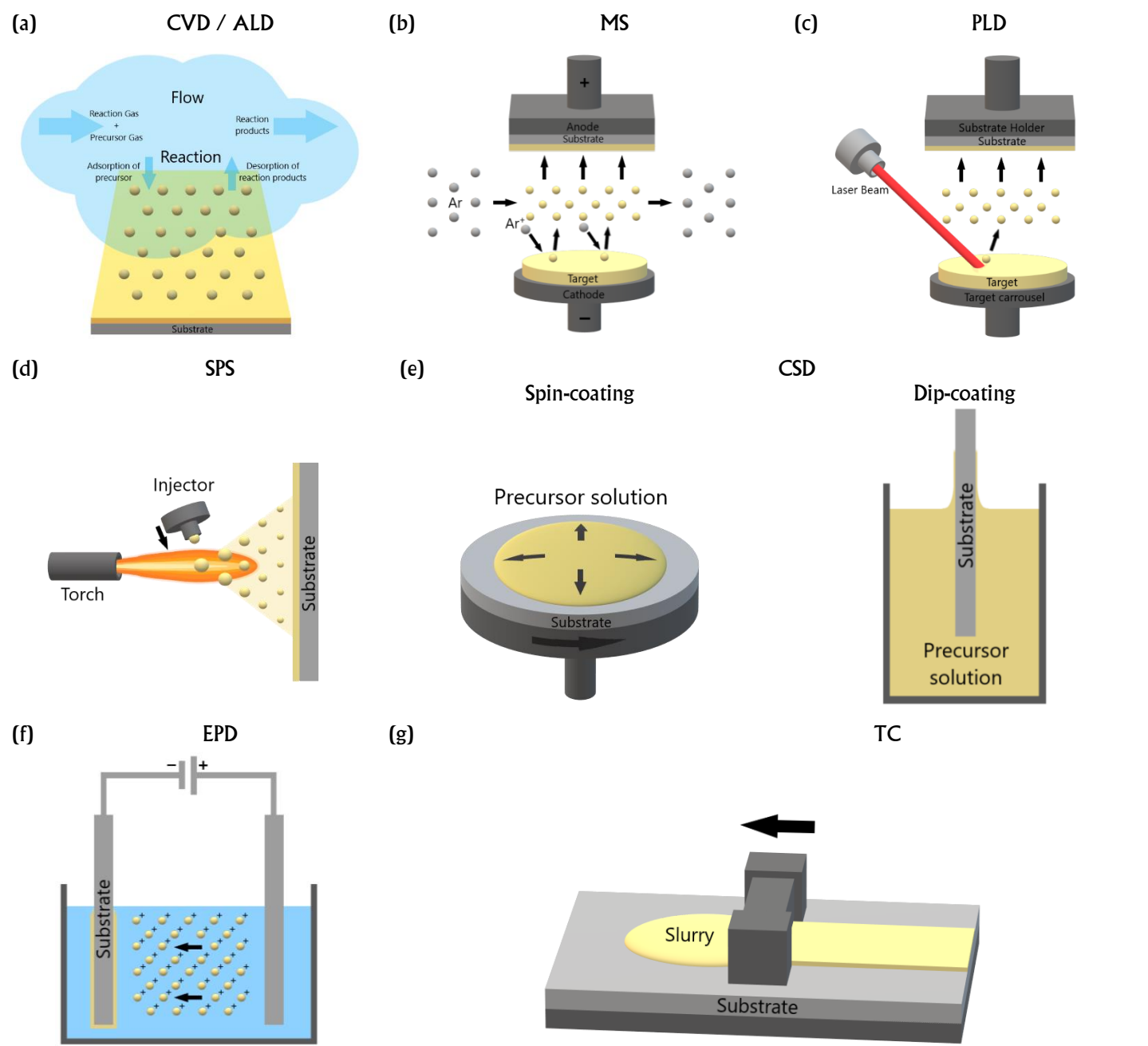
Figure 1 Schemes of different methods of thin-film formation.
