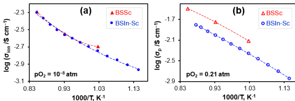
Figure 8 Temperature dependences of electrical conductivity of \text{BaSn}_{0.7}\text{In}_{0.15}\text{Sc}_{0.15}\text{O}_{3-\delta} (BSIn-Sc) vs. \text{BaSn}_{0.7}\text{Sc}_{0.3}\text{O}_{3-\delta} (BSSc) [19] ceramic samples: (a) ionic conductivity, (b) hole conductivity.
