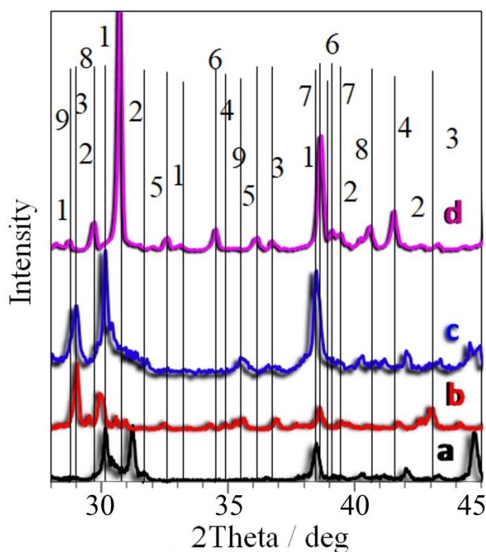
Figure 7 Diffraction patterns of the studied oxide-fluoride mixtures after \text{ZrO}_2 dissolution.
