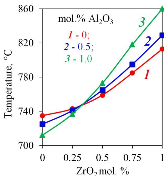
Figure 4 Liquidus temperatures of \text{KF-NaF-AlF}_3 melts depending on the content of \text{ZrO}_2 and \text{Al}_2\text{O}_3 ( [\text{KF}] + [\text{NaF}]/[\text{AlF}_3] = 1.3 ).
