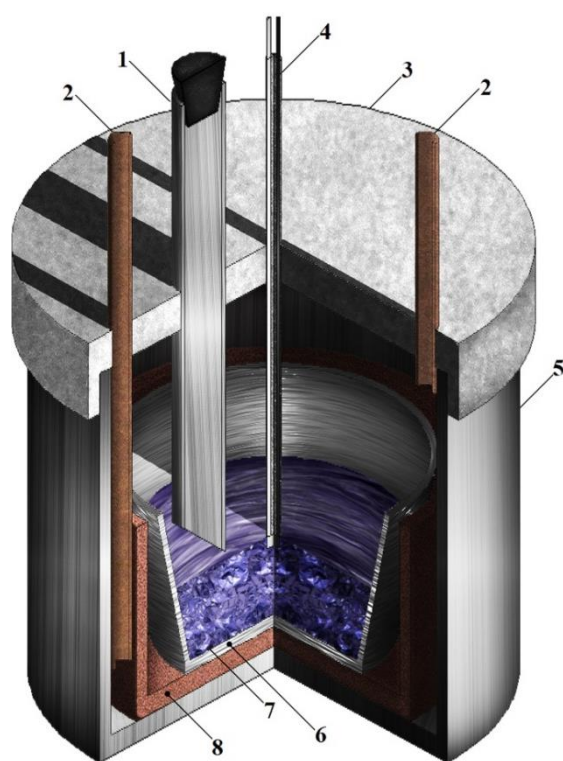
Figure 1 Diagram of the experimental cell for measuring the liquidus temperatures of the studied melts with \text{ZrO}_2 and \text{Al}_2\text{O}_3 additives: 1 – quartz tube; 2 – alundum tube; 3 – fluoroplastic cover; 4 – thermocouple; 5 – quartz retort; 6 – platinum crucible; 7 – melt under study; 8 – protective alundum glass.
