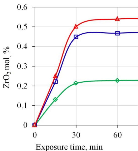
Figure 3 \text{ZrO}_2 content in the \text{NaF-AlF}_3 melt ( [\text{NaF}]/[\text{AlF}_3] = 1.3 ) at 750 °C after adding \text{ZrO}_2 in the amount of wt. % (mol. %): \diamond – 0.5 (0.28), \square – 1.0 (0.56), \Delta – 1.5 (0.84).
