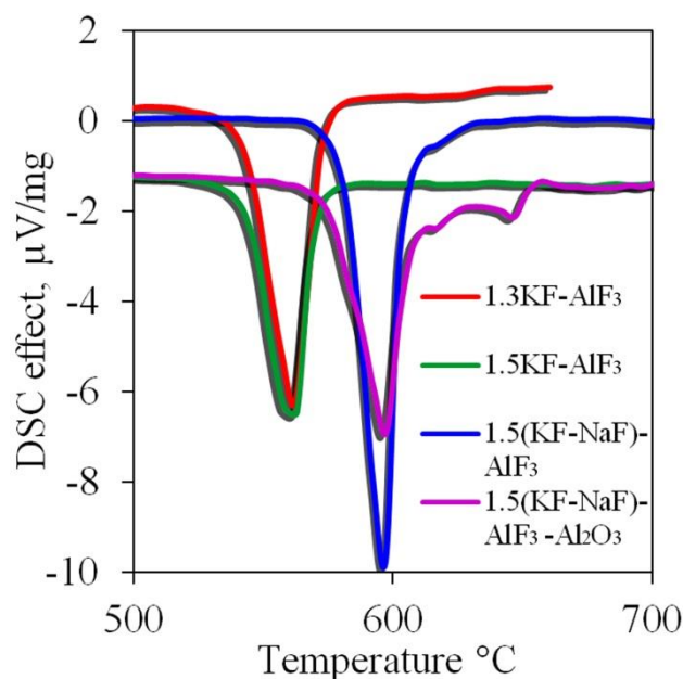
Figure 5 Thermal effects in the mixtures of \text{KF-AlF}_3 , \text{KF-NaF-AlF}_3 and \text{KF-NaF-AlF}_3\text{-Al}_2\text{O}_3 with the addition of 1.0 mol. % \text{ZrO}_2 when heated to 800 °C.
