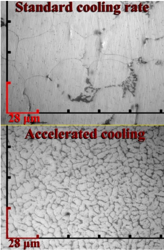
Figure 7 Microphotographs of the AK6 alloy without zirconium additives, obtained at different cooling rates: 1 – standard; 2 – 10 3 K/s.
