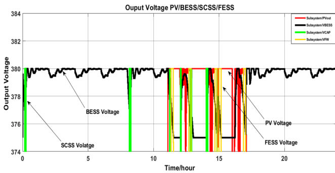
Figure 4. PV/BESS/SCSS/FESS output
