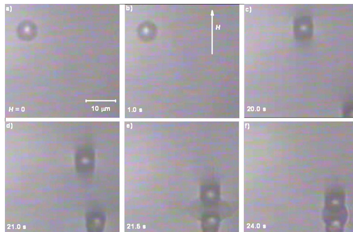
Figure 1. Snapshots of the aggregation of two nickel particles dispersed in a ferrofluid, upon application of a magnetic field of 22 kA/m. Direction of the field is indicated. Ferrofluid solid concentration was 5 % vol. Snapshot a) was taken prior to magnetic field application. Snapshots b) to f) were taken after field application. Time elapsed since field application is indicated in each snapshot.
