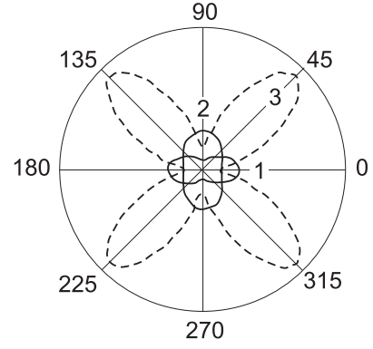
FIG. 4: The absorption coefficient K(\omega, \varphi) , eq.(23), at selected frequencies as a function of polarization angle \varphi . 1: \omega = \omega_1 . 2: \omega = \omega_2 . 3: \omega = \omega_3 (see text).
