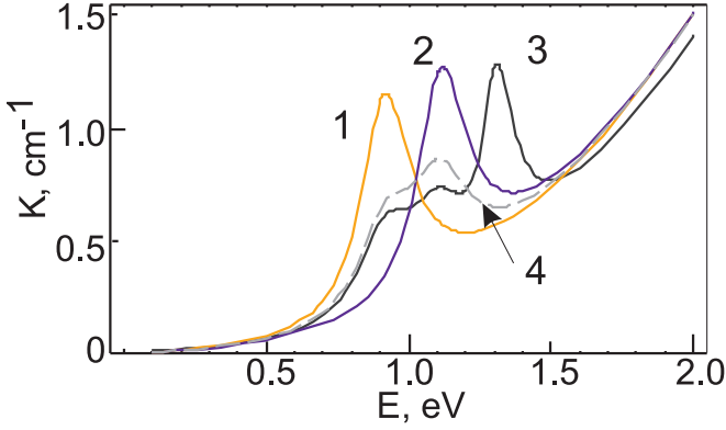
FIG. 3: The absorption coefficient, obtained with eqs.(23,24). Curves 1 and 2 depict the response in two plane polarizations, \varphi = 0 and \varphi = \pi/2 , respectively. The curve 3 simulates the spectrum, obtained in unpolarized light. Noteworthy is the novel peak at 1.3 eV, not observed in two previous polarizations. The dashed curve 4 is the unpolarized light spectrum of a conventional medium and is obtained using the trivial counterpart of the dielectric tensor, eq.(20), where the angle-dependent terms are omitted.
