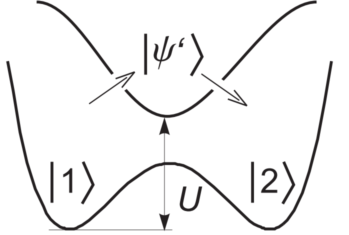
FIG. 2: Schematic picture of the optical switching transition. The center is excited from its ground state |1\rangle to the intermediate state |\psi'\rangle , absorbing the photon with polarization p_1 , and then may either relax back to its initial state or switch to another ground state |2\rangle .
