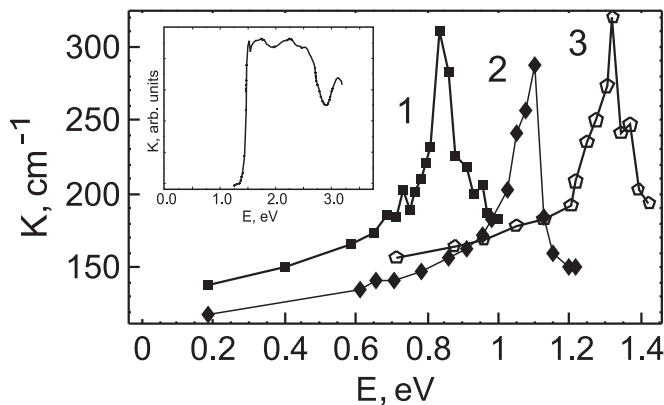
FIG. 1: The absorption spectra of CuO sample after the bombardment with \text{He}^+ nuclei 1 . Spectra 1 and 2 are obtained in plane polarizations \mathbf{E} \parallel [\bar{1}01] and \mathbf{E} \perp [\bar{1}01] , respectively. Spectrum 3 is obtained in unpolarized light. Solid lines are guides to the eye. Inset: the absorption spectra of CuO high quality single crystal.
