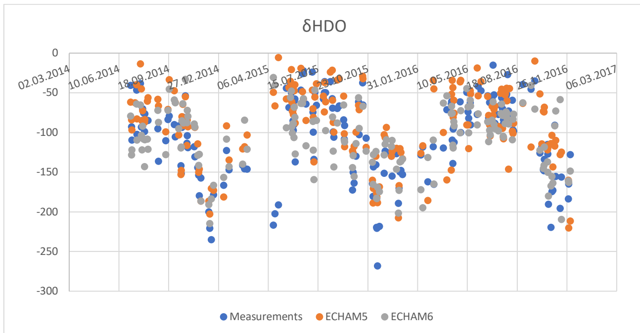
Fig. 2 – Comparison of model and measured data on \delta\text{HDO} in precipitation collected at a monitoring station in the foothills of the Altai
