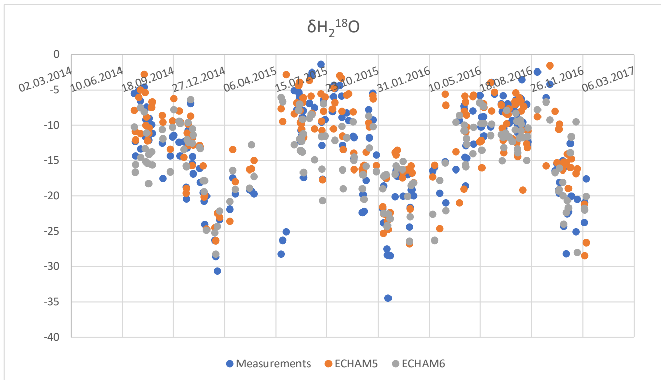
Fig. 1 – Comparison of model and measured data on \delta\text{H}_2^{18}\text{O} in precipitation collected at a monitoring station in the foothills of the Altai
