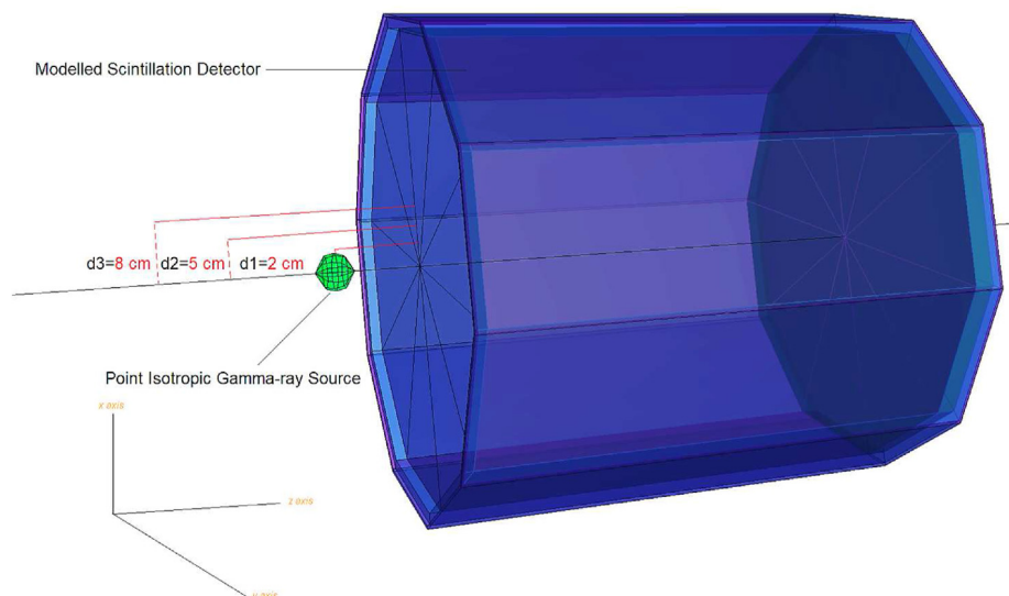
Figure 2. 3-D view of modeled detector setup and distances of source in MCNPX (version 2.6.0) provided by MCNPX Visual Editor (visedX22S).
