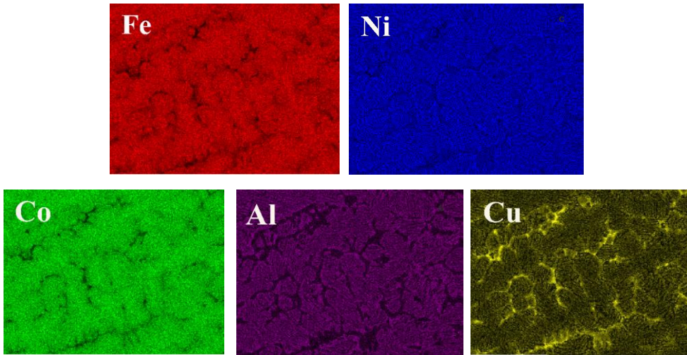
Fig. 3 EDS elemental map of equiatomic AlFeCoNiCu
