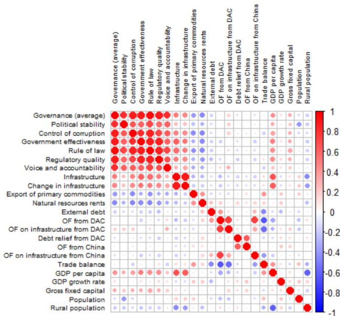
Figure A1. Correlation matrix plotted a circle diagram with the colour and the size of circles illustrating the sign and the absolute size of the correlations.
