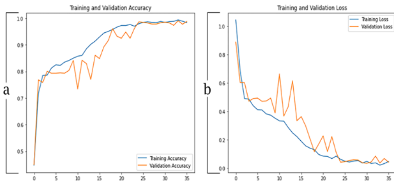
Fig. 5. Accuracy and loss graphs during model trainings: (a) training and validation accuracy; (b) training and validation loss
