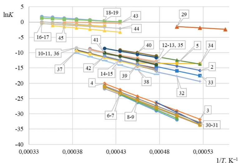
Figure 4. Equilibrium constants of reactions as a function of 1/T in the process of radioactive graphite heating in air at T = 1900 – 2900 K.
