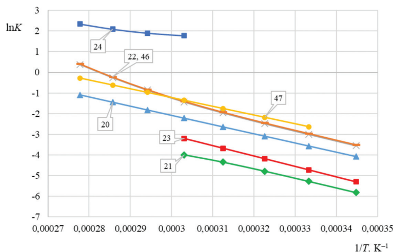
Figure 5. Equilibrium constants of reactions as a function of 1/T in the process of radioactive graphite heating in air at T = 2900 – 3600 K.
