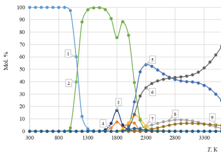
Figure 2. Distribution of calcium by equilibrium phases in the process of radioactive graphite heating in air: 1 – CaCl_{2(c)} ; 2 – CaCl_2 ; 3 – CaUO_{4(c)} ; 4 – CaO ; 5 – Ca ; 6 – Ca^+ ; 7 – CaCl ; 8 – CaO ; 9 – CaO^+ ; 10 – CaCl^+ .
