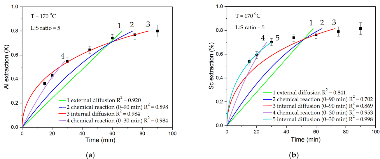
Figure 5. The results of fitting data (points) to different equations of shrinking core model (SCM) (lines): (a) extraction of Al; (b) extraction of Sc.
