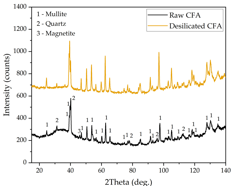
Figure 1. XRD patterns of the Reftinskaya TPP coal fly ash (CFA) and coal fly ash after desilication (DCFA).
