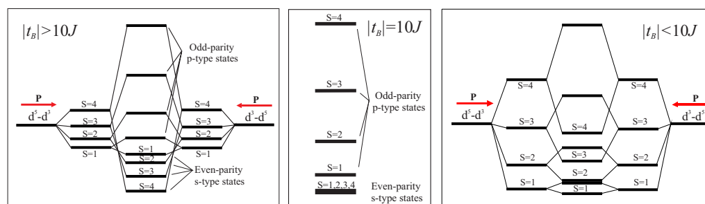
Figure 1. (Color online): Spin structure of the EH dimer, or self-trapped CT exciton with a step-by-step inclusion of the one- and two-particle charge transfer. Arrows point to electric dipole moments for bare site-centered dimer configurations.
