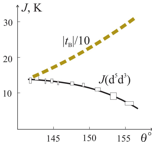
Figure 2. (Color online): Angular dependencies of J(d^5 d^3) and \frac{1}{10}|t_B| , which define the effective integral J_{eff} = J(d^5 d^3) - 0.1|t_B| .
