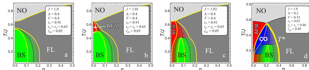
Figure 3. (Color online): Model phase T - n -diagrams of hole-doped \text{CuO}_2/\text{NiO}_2 planes in cuprates/nickelates calculated in the effective field approximation ( n = p for hole doping), with the phase separation taken into account using Maxwell's construction; J is the exchange integral, \Delta = U/2 is the local correlation parameter, V is the nonlocal correlation parameter, t_p , t_n , t_{pn} are three independent integrals of the correlated single-particle transfer, t_B is the effective transfer integral of the composite boson (see insets), assuming competition between “monophases” NO (disordered), AFMI, BS, FL, and CO. The boundaries between the phases represent lines of equal free energies. The dashed curves (a–d) indicate the lines of equal volume fractions of two neighboring phases, the yellow curves represent the lines of phase transitions of the “third” kind, limiting the regions with maximal 100% volume fractions of one of the phases. See Refs. [43,44] for more details. Pay attention to the strong change in the phase diagram, even with a very small change in the parameters of the Hamiltonian (compare panels a–c).
