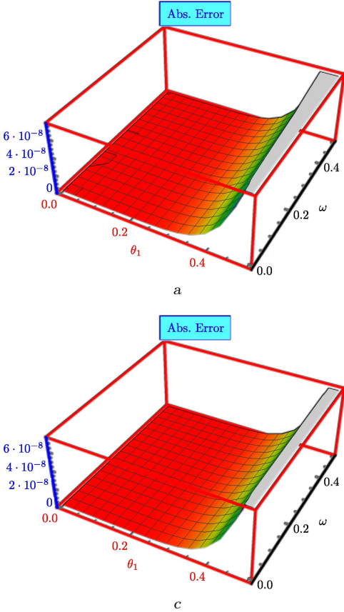
Figure 4. The 3D plots of the Abs-E of \aleph(\theta_1, \omega) (a), \aleph(\theta_1, \theta_2, \theta_3, \omega) (b), and \aleph(\theta_1, \theta_2, \omega) (c) for the approximate finding obtained through seven iterations and exact result in the ranges \omega \in [0, 0.5] and \theta_1 \in [0, 0.5] , when \theta_2 = \theta_3 = 0.25 (b), and \theta_2 = 0.25 (c)
