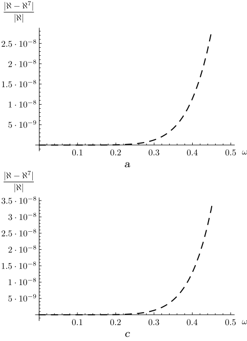
Figure 3. The 2D curves of the Rel-E graph of \aleph(\theta_1, \omega) (a), \aleph(\theta_1, \theta_2, \theta_3, \omega) (b), and \aleph(\theta_1, \theta_2, \omega) (c) for the approximate finding obtained through seven iterations and the exact result in the range \omega \in [0, 0.5] , when \theta_1 = 0.25 (a), \theta_1 = \theta_2 = \theta_3 = 0.25 (b), and \theta_1 = \theta_2 = 0.25 (c)
