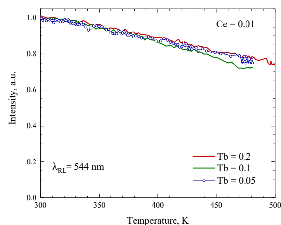
Figure 5. Normalized temperature dependence of the XRL intensity at the registration at 544 nm for samples with an optimal Ce content. Concentrations of Ce and Tb indicated.
