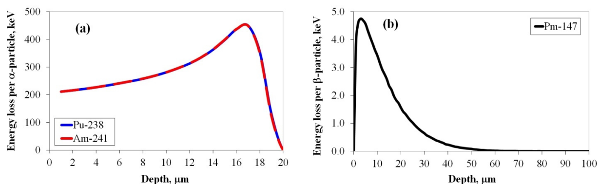
Figure 9. Energy loss profile for \alpha -particles (a) and \beta -particles (b) of specified isotopes in (\text{Gd,Y,Tb,Ce})_3\text{Al}_2\text{Ga}_3\text{O}_{12} converter material.
