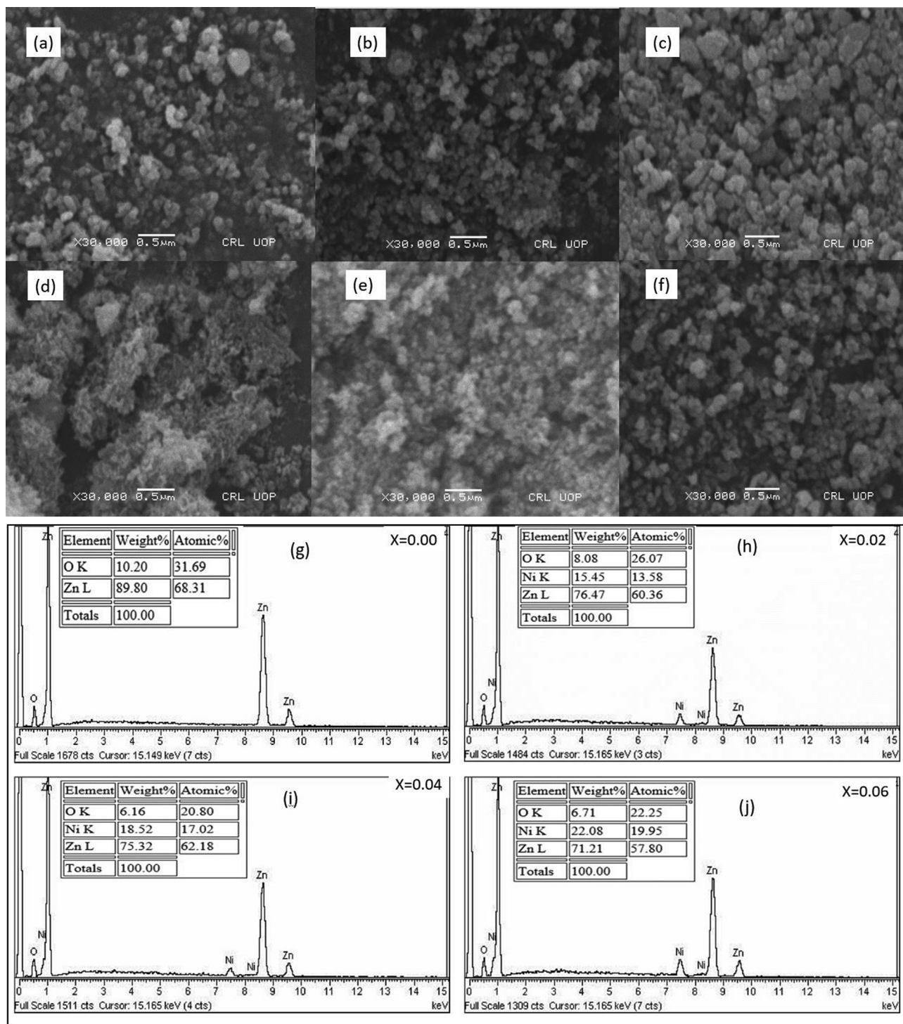
Fig. 2. SEM and EDX results of \text{Zn}_{1-x}\text{Ni}_x\text{O} NPs (a) x = 0.00 at pH = 9 (b) x = 0.02 at pH = 9 (c) x = 0.04 at pH = 9 (d) x = 0.06 at pH = 9 (e) x = 0.04 at pH = 11 (f) x = 0.04 at pH = 13 (g) x = 0.00 at pH = 9 (h) x = 0.02 at pH = 9 (i) x = 0.04 at pH = 9 (j) x = 0.06 at pH = 9.
