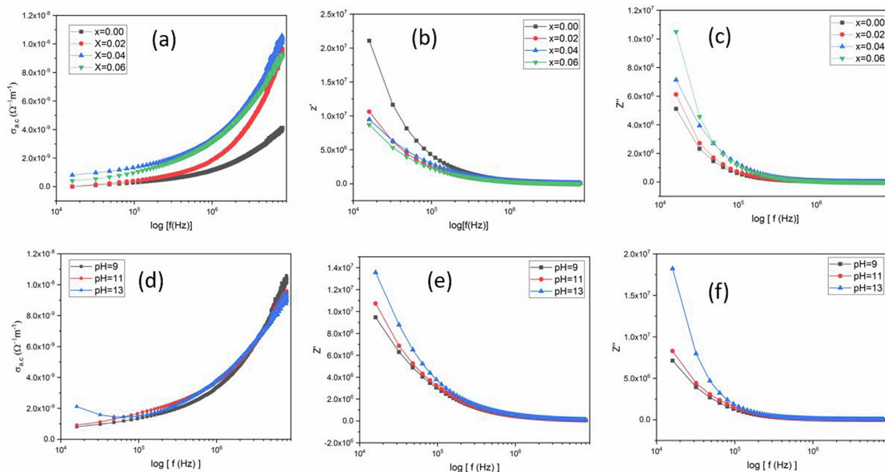
Fig. 6. Frequency dependence AC properties of \text{Zn}_{1-x}\text{Ni}_x\text{O} (a) AC conductivity, (b) Impedance real part, (c) Impedance imaginary part, for variant concentration and (d) AC conductivity (e) Impedance real part (f) impedance imaginary part, at different pH.
