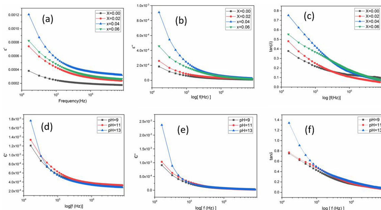
Fig. 5. Frequencies dependent dielectric properties of \text{Zn}_{1-x}\text{Ni}_x\text{O} NPs (a) real (b) imaginary (c) lose factor, for variant concentration and (d) real (e) imaginary (f) lose factor, at different pH.
