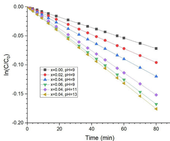
Fig. 10. Photocatalytic degradation (%) of MO dye followed pseudo-first order kinetics.
