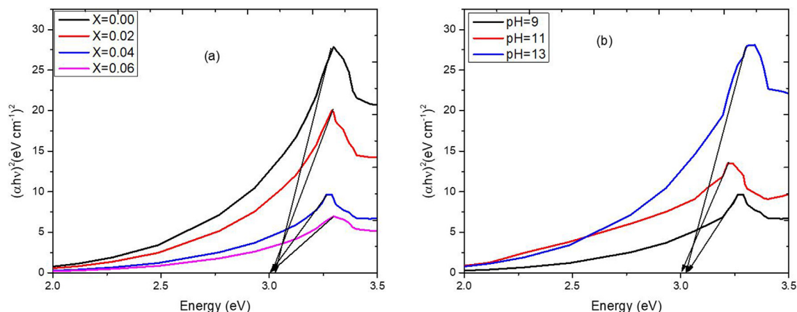
Fig. 3. Tauc plot of \text{Zn}_{1-x}\text{Ni}_x\text{O} NPs at varying (a) concentration (b) pH.
