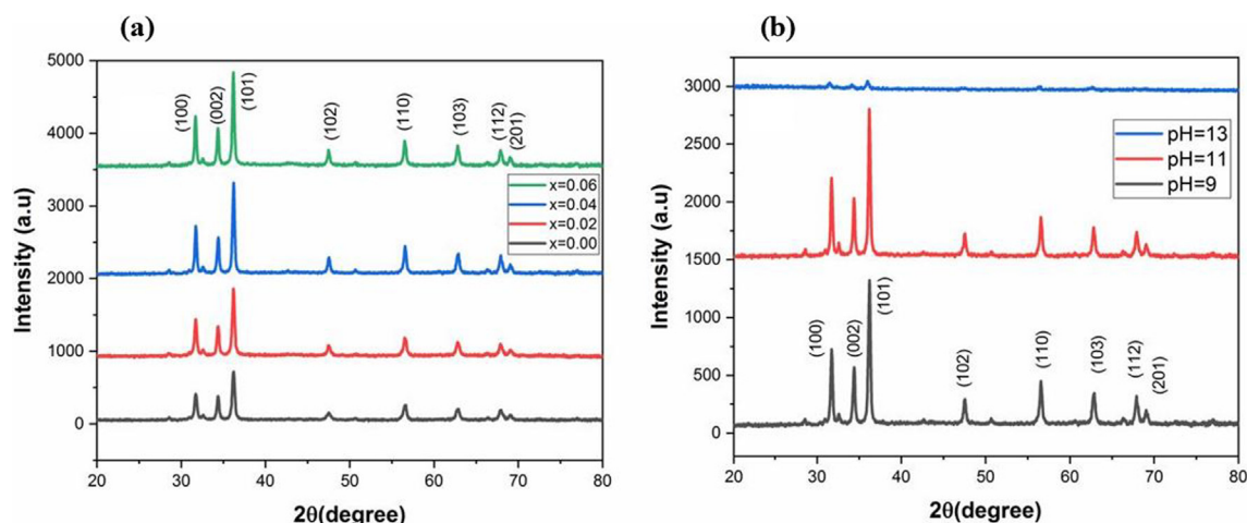
Fig. 1. The XRD pattern of Ni doped ZnO NPs at varying (a) dopant concentration (b) pH.
