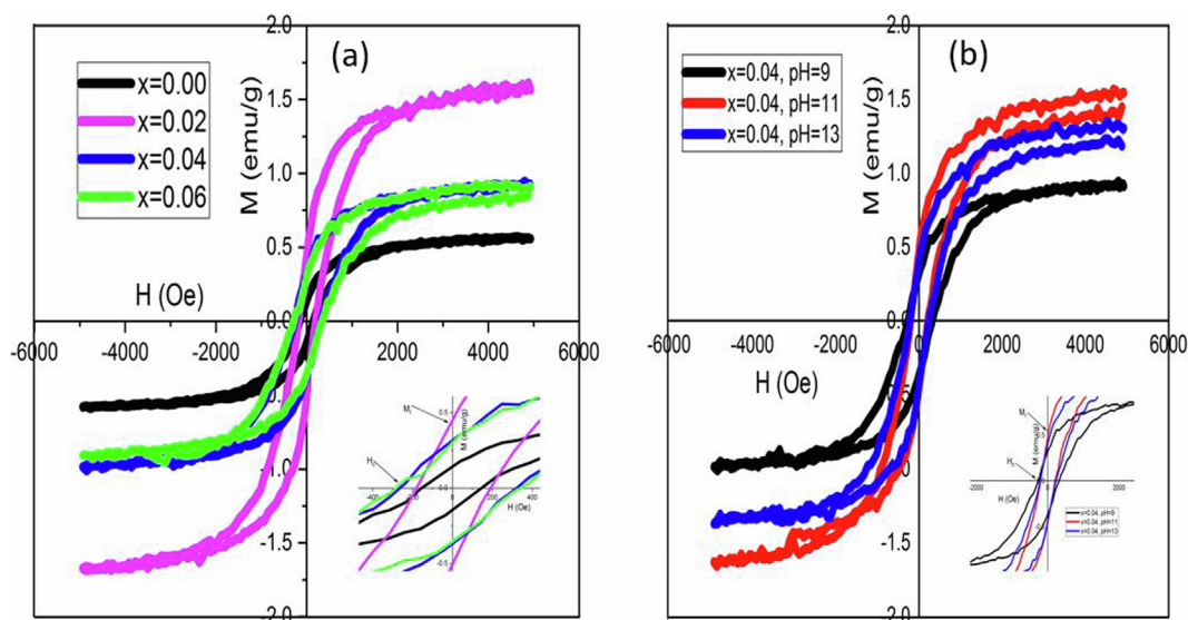
Fig. 7. Magnetic hysteresis (M–H) loops of the \text{Zn}_{1-x}\text{Ni}_x\text{O} NPs for (a) concentration (b) pH.
