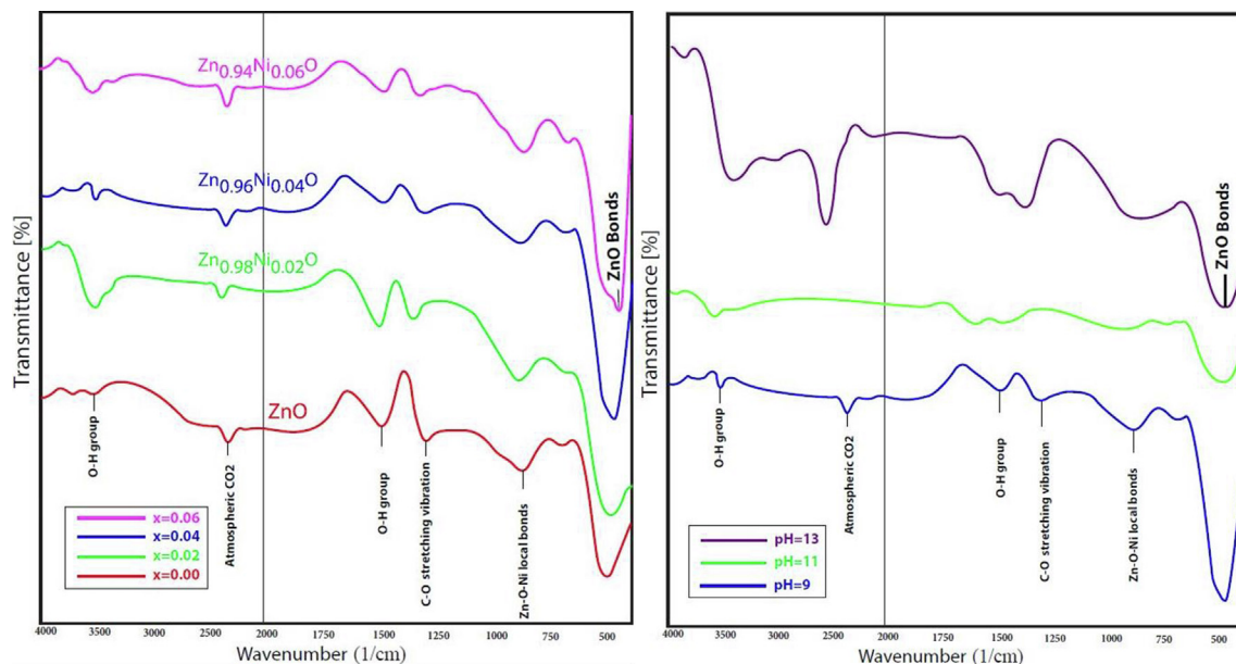
Fig. 4. FTIR spectra of Ni doped ZnO NPs synthesized at varying (a) concentration (b) pH.
