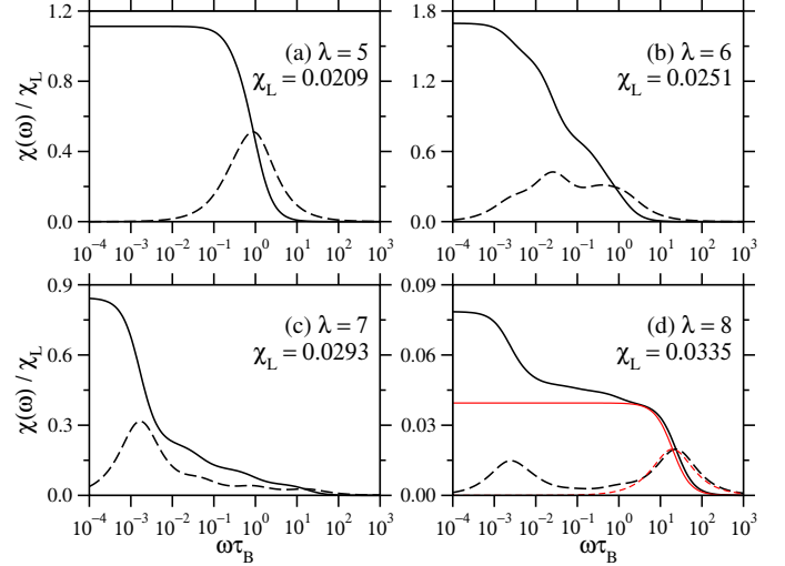
Figure 3: The dynamic magnetic susceptibility \chi(\omega) , divided by the Langevin susceptibility \chi_L , for ferrofluids with volume fraction \varphi = 5.24 \times 10^{-4} : (a) \lambda = 5 ; (b) \lambda = 6 ; (c) \lambda = 7 ; (d) \lambda = 8 . The solid black line represents the real part, and the dashed black line the imaginary part, from BD simulations. In (d), the solid red line and dashed red line represent the Debye functions with an effective Brownian time 0.0510\tau_B , and scaled to give the peak height in \chi''(\omega) .
