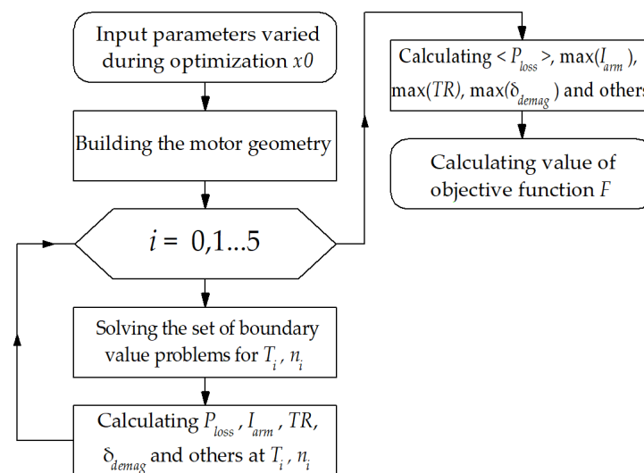
Figure 5. Objective function calculation block diagram.
