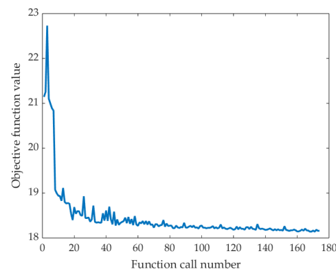
Figure 12. FaSynRM optimization progress.
