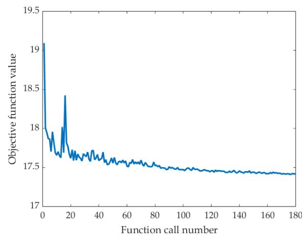
Figure 7. FaSHM optimization progress.
