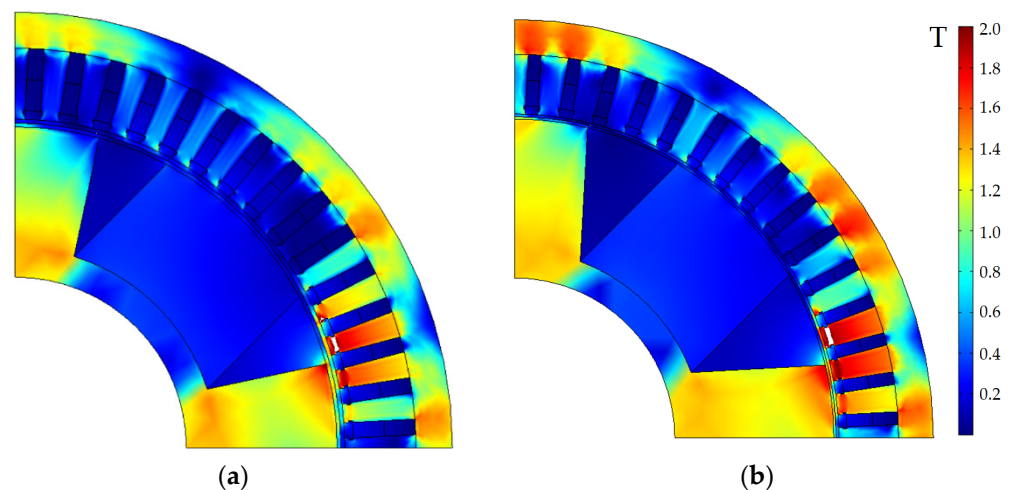
Figure 8. The cross-section of the optimized designs of the FaSHM and the plot of flux density magnitudes at operating point 4; saturation areas ( >2 T) are shown with white. (a) Design optimized in [14]; (b) New FaSHM design.
