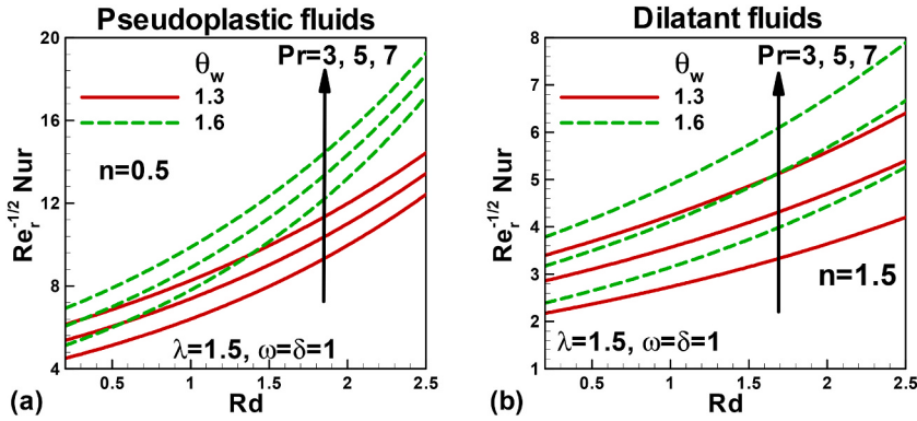
Fig. 10. (a, b): Alteration of Nusselt number with radiation parameter for diverse fluids and temperature ratio.
