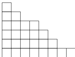
Figure 1. The Ferrers diagram of the partition (6, 5, 4, 4, 3, 2, 1, 1) .
