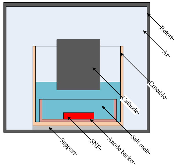
Fig. 7. Schematic image of an electrolytic refinery apparatus along the Oz axis.
