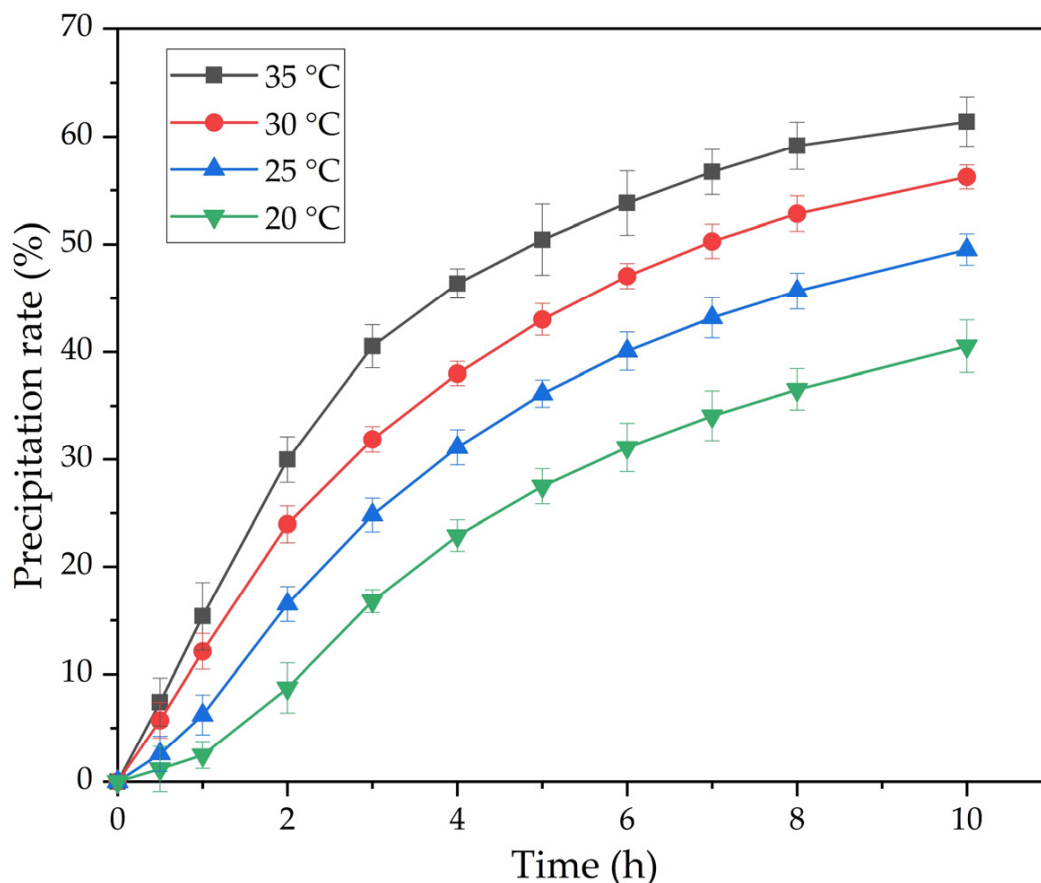
Figure 6. The effect of temperature and time on the precipitation of the flake-like gibbsite (FLG) from an alkaline aluminate solution ( \text{Na}_2\text{O}_k = 150 \text{ g L}^{-1} , \alpha_k = 1.5 ) using active aluminum hydroxide in the amount of 20 \text{ g L}^{-1} as a seed.
