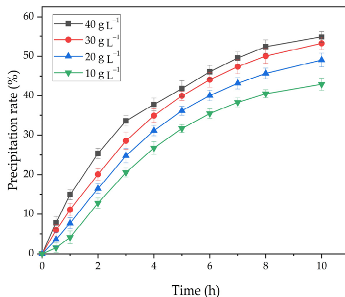
Figure 9. The effect of the duration and amount of active seed on the degree of precipitation at 25^\circ\text{C} and the \text{Na}_2\text{O} concentration 150 \text{ g L}^{-1} .
