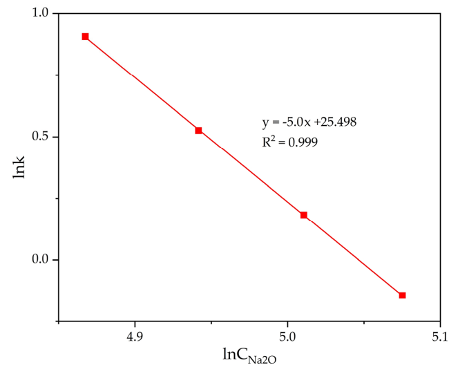
Figure 14. Dependence of \ln K - \ln C_{\text{Na}_2\text{O}} (Table 3) for the precipitation of FLG from an aluminate solution at various \text{Na}_2\text{O}_k concentration.
