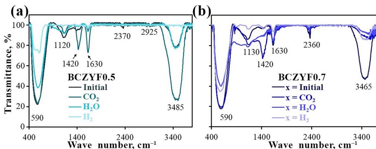
Figure 9 IR spectra of the samples with BCZYFo.5 (a) and BCZYFo.7 (b) compositions after their treatments in different atmospheres at 1100 °C for 10 h.
