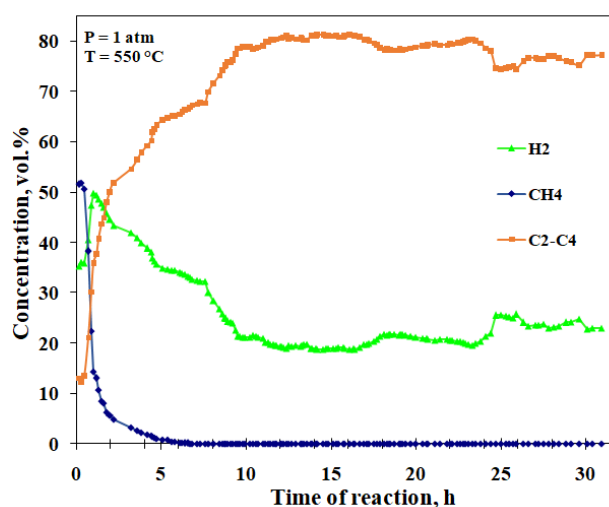
Figure 2 Change in the volume concentrations of the reaction products depending on the reaction time (1 atm, 550 °C).
