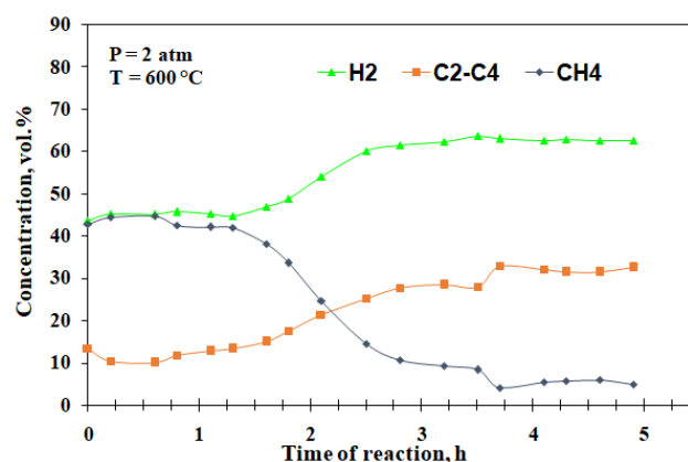
Figure 4 Change in the volume concentrations of the reaction products depending on the reaction time (2 atm, 600 °C).
