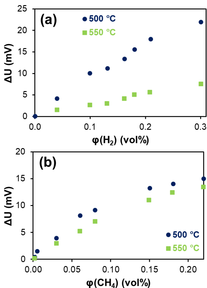
Figure 4 Mixed potential value between Pt- and ZnO-based electrodes depending on (a) the hydrogen content in \text{O}_2 + \text{H}_2 + \text{N}_2 gases and (b) the methane content in \text{O}_2 + \text{CH}_4 + \text{N}_2 gases.
