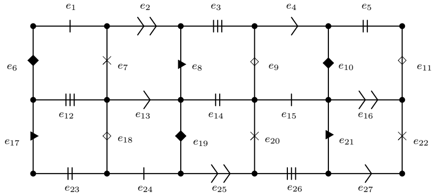
Figure 7. \mathcal{P}_3(K_2)(P_3 \times P_6) .
