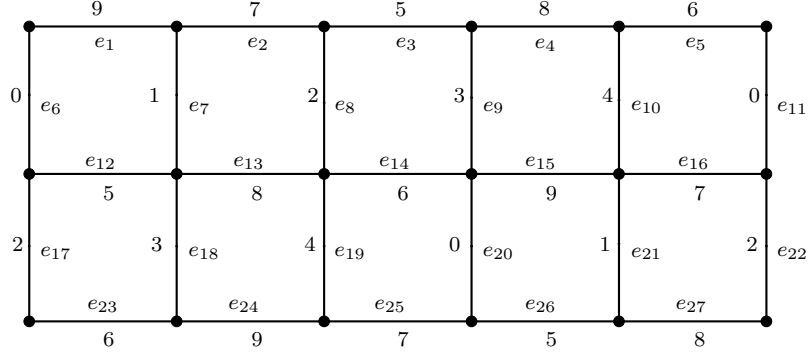
Figure 6. Optimal L'(2,1) -edge coloring of P_3 \times P_6 .
