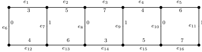
Figure 2. Optimal L'(2, 1) -coloring of P_2 \times P_6 .
