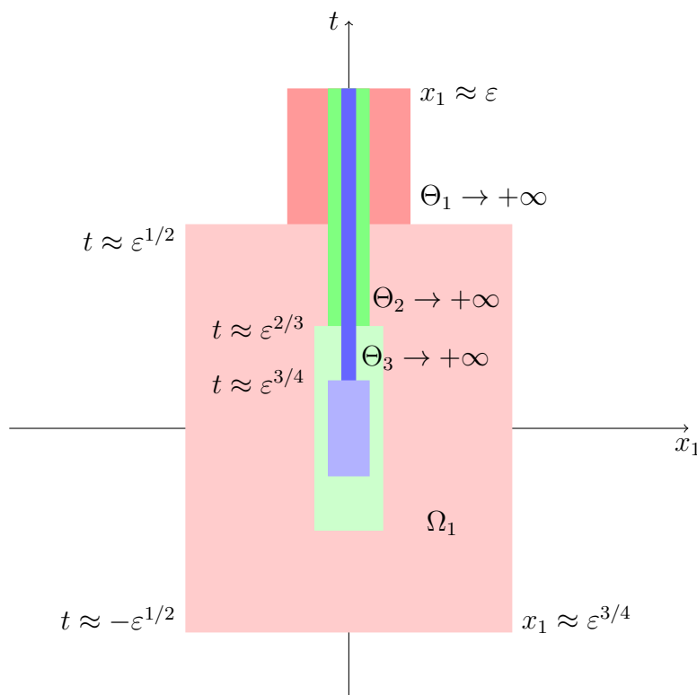
Figure 3. A schematic projection of the domain of the localization of the singularity in the plane (x_1, t) .
