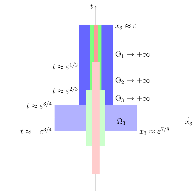
Figure 1. A schematic projection of the domain of the localization of the singularity in the plane (x_3, t) .
