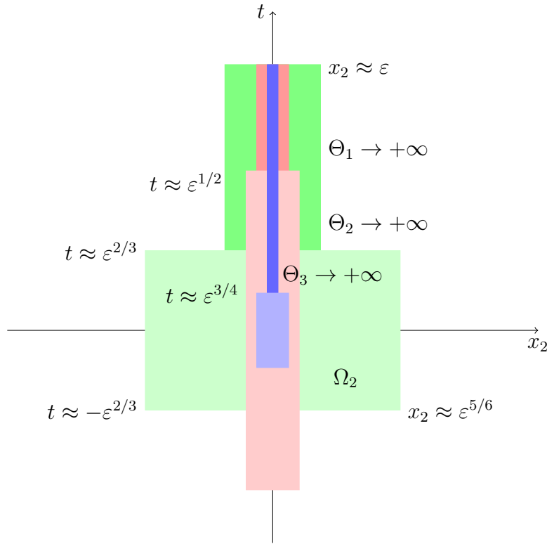
Figure 2. A schematic projection of the domain of the localization of the singularity in the plane (x_2, t) .
