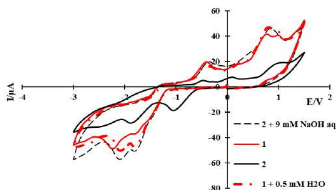
Figure 5 CV curves of 5 mM compounds 1,2 in DMF (0.1 M \text{Bu}_4\text{NBF}_4 ), recorded using GCE with v = 0.1 V/s: red – 1, red dotted line – 1 with the addition of 0.5 mM \text{H}_2\text{O} , black – 2, black dotted line – 2 with the addition of 9 mM aqueous NaOH.
