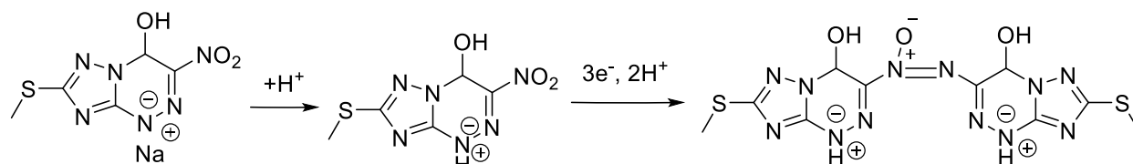
Figure 6 Probable mechanism of electrochemical reduction of compound 1 in BRB pH = 2.
