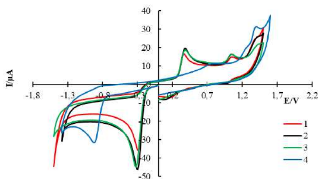
Figure 2 CV curves of 1 mM compounds 1–4 : in BRB pH = 2 using GCE at v = 0.1 V/s. Potentials were measured relative to Ag/AgCl/KCl sat .
