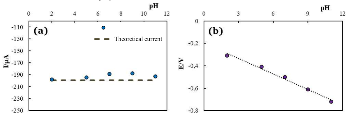
Figure 3 Values of current (A) and potential (B) of the peak of compound 1 (5 mM) with a change in the pH of the buffer solution at v = 100 mV/s.
