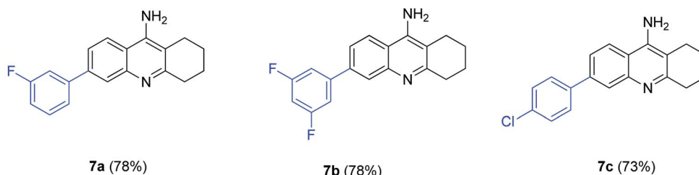
Scheme 2 Synthesis of 6-arylated tacrine derivatives by Suzuki–Miyaura coupling; reaction conditions: 6-borylated tacrine (1 mmol), aryl bromide (1.2 mmol), \text{Pd}(\text{dppf})\text{Cl}_2 \cdot \text{CH}_2\text{Cl}_2 (5 mol%), \text{K}_2\text{CO}_3 (2.5 mmol), 1,4-dioxane (2 mL), \text{H}_2\text{O} (1 mL), 100 °C for 8–10 h.
