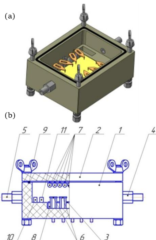
Figure 3 Model of measurement cell for the characterization of gas sensors (a) and its scheme (b): housing (1), cover (2), common contact (3), gas inlet connection (4), gas outlet connection (5), clamping contacts (6), LEDs (7), heater (8), sealing (9), humidity-temperature sensor (10), pressure sensor (11).
