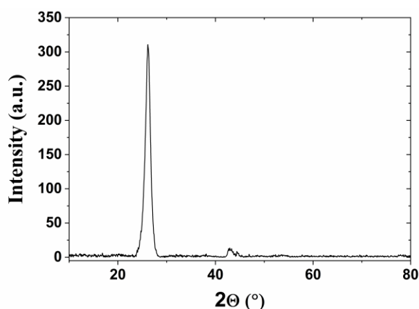
Figure 6 X-ray diffraction pattern of MWNTs.
