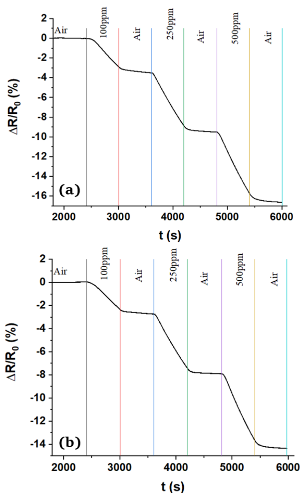
Figure 8 Response of MWNT pellets compacted under 9 MPa (a) and 13 MPa (b) pressure to 100–500 ppm NO 2 at room temperature.
