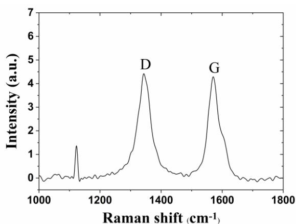
Figure 5 Raman spectrum of MWNTs.
