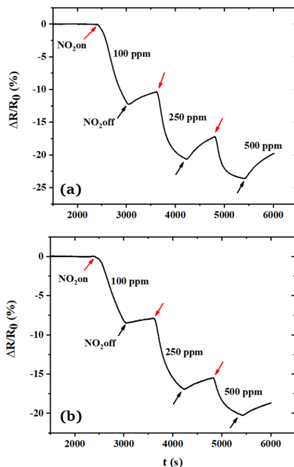
Figure 7 Response of MWNT films obtained in ethanol (a) and in acetone (b) to 100–500 ppm \text{NO}_2 at room temperature.
