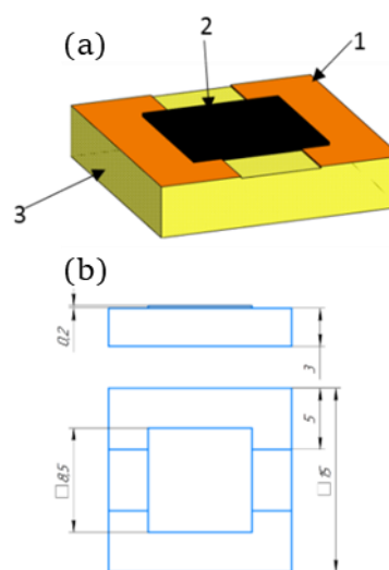
Figure 1 Obtained sensor (a): copper contacts (1), film of CNMs (2), dielectric substrate (3) and its scheme (b).
