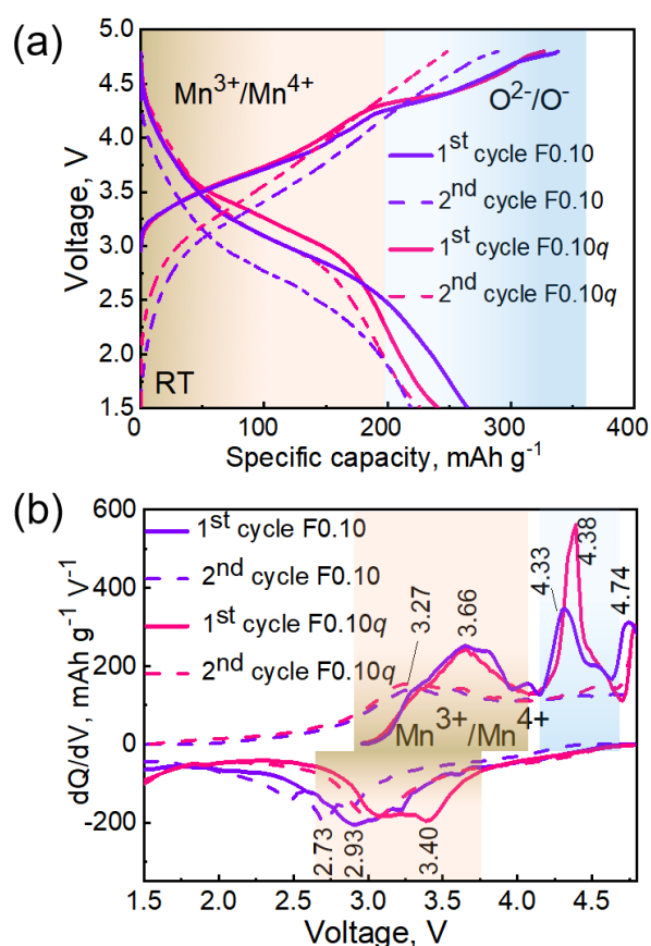
Figure 6 Charge-discharge curves of the Fo.10 and Fo.10q samples, cycled at the C/40 charge/discharge rate within the voltage range of 1.5–4.8 V at RT (a) and corresponding dQ/dV curves (b).
