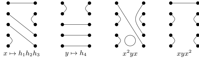
Fig. 7. The identity x^2yx \simeq xyx^2 fails in \mathcal{K}_5
