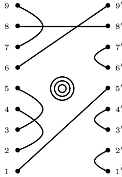
Fig. 1. Wire diagram representing an element of \mathcal{W}_9
