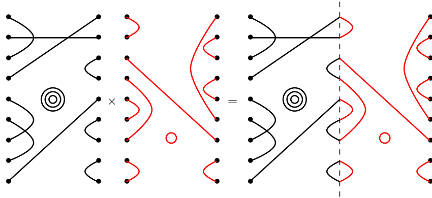
Fig. 2. Multiplication of wire diagrams
