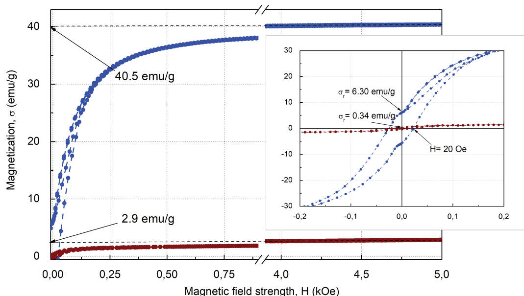
Figure 4: Part of the magnetic hysteresis loops in an extended range and the same data in a limited range measured at T = 300 K for samples of magnetized RM (blue) and initial RM (brown); H – coercive force, Oe; \sigma_r – residual magnetization, emu/g.
