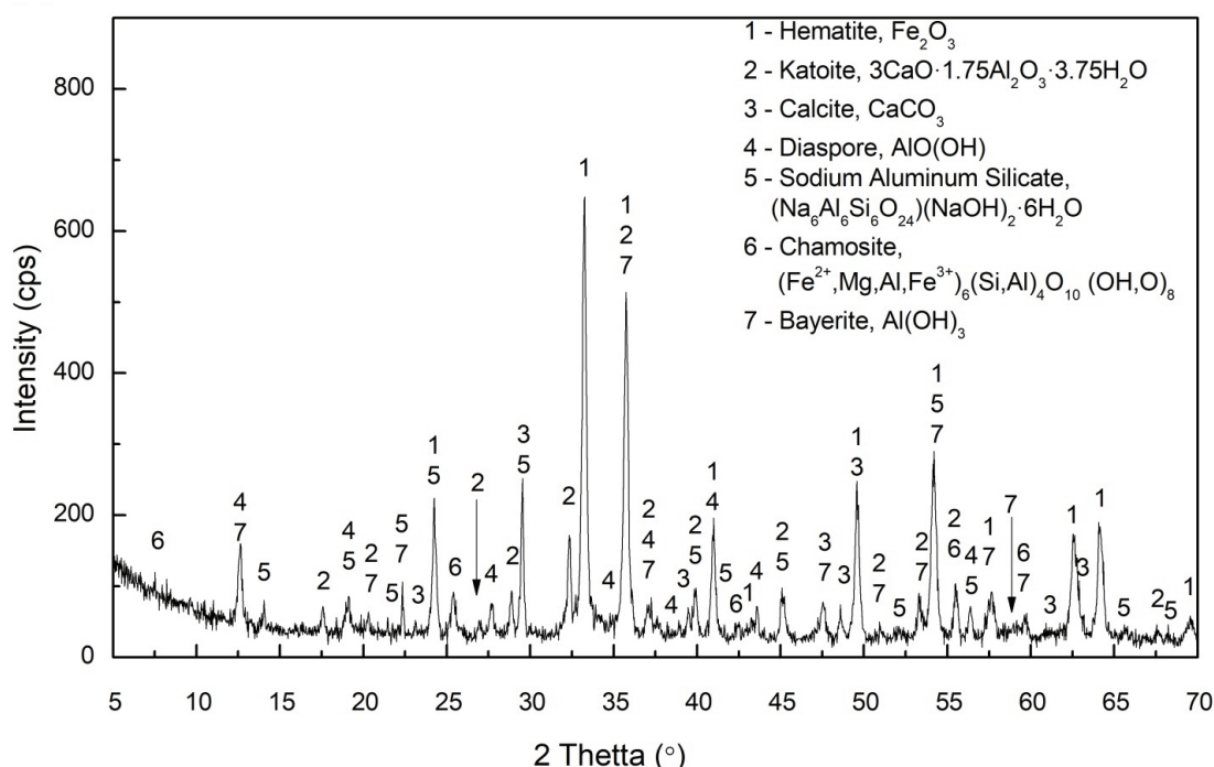
Figure 1: The XDR pattern of initial RM.
