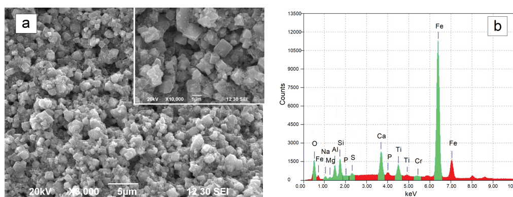
Figure 3: a – SEM image of magnetized RM with a magnification of \times 3000 (in the insert \times 10\,000 ), b – EDX-spectra for the selected region
