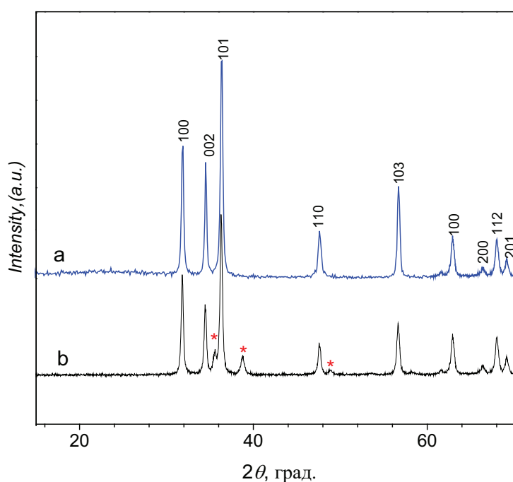
Figure 2: X-ray diffraction patterns of Zn_{1-x}Cu_xO samples: a - x = 0.05 ; b - x = 0.2 ; CuO - (*)
