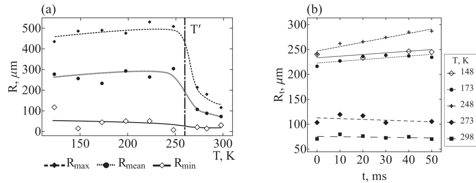
Figure 2: Temperature dependence of averaged over time, minimum and maximum spiral dynamic domains radii R ; (b) averaged spiral dynamic domains radius R_i vs time t counted from their nucleation for several film temperatures.
